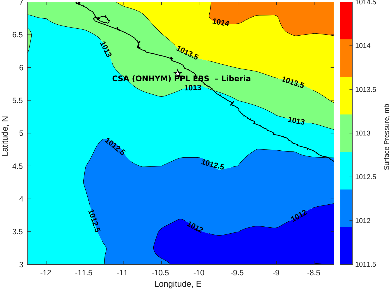
Surface Pressure (mb) for CSA (ONHYM) PPL EBS - Liberia at 03-May-2025 00:00:00
