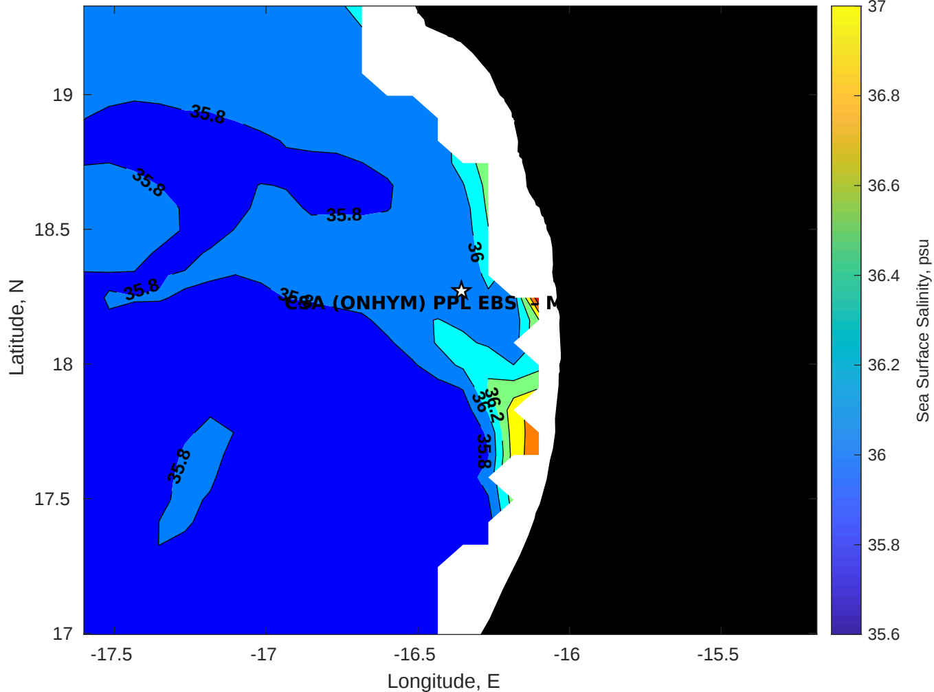
Surface Salinity for CSA (ONHYM) PPL EBS - Mauritania at 02-May-2025 00:00:00
