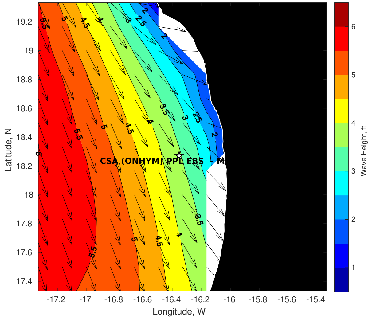
Wave Height (ft) for CSA (ONHYM) PPL EBS - Mauritania at 03-May-2025 09:00:00
