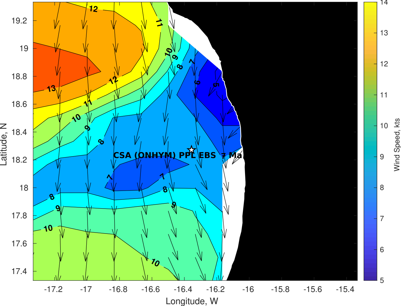
Winds (kts) for CSA (ONHYM) PPL EBS - Mauritania at 03-May-2025 09:00:00
