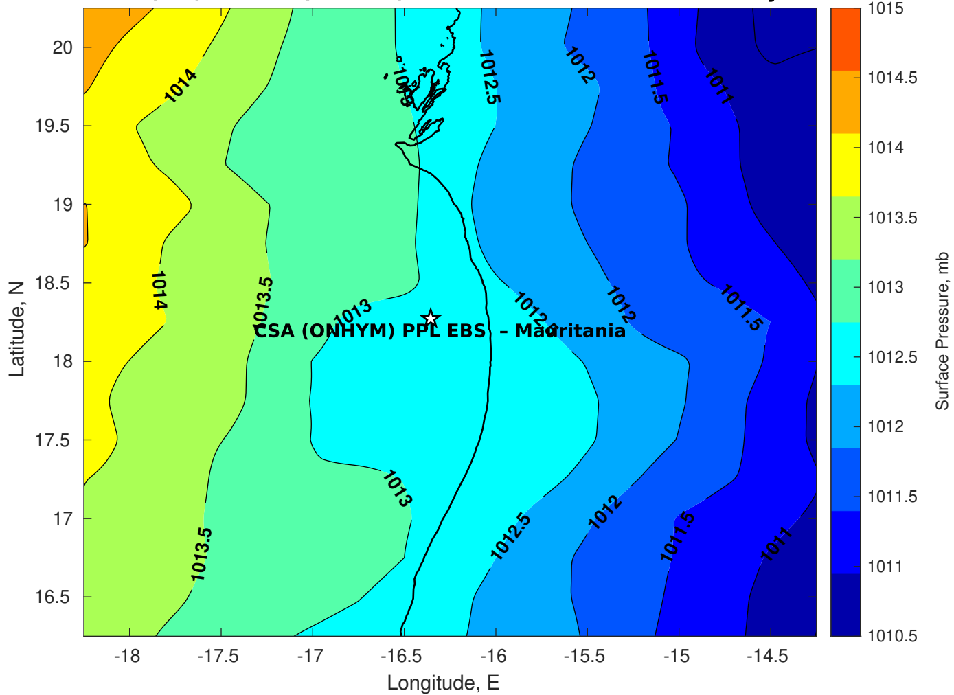
Surface Pressure (mb) for CSA (ONHYM) PPL EBS - Mauritania at 05-May-2025 00:00:00
