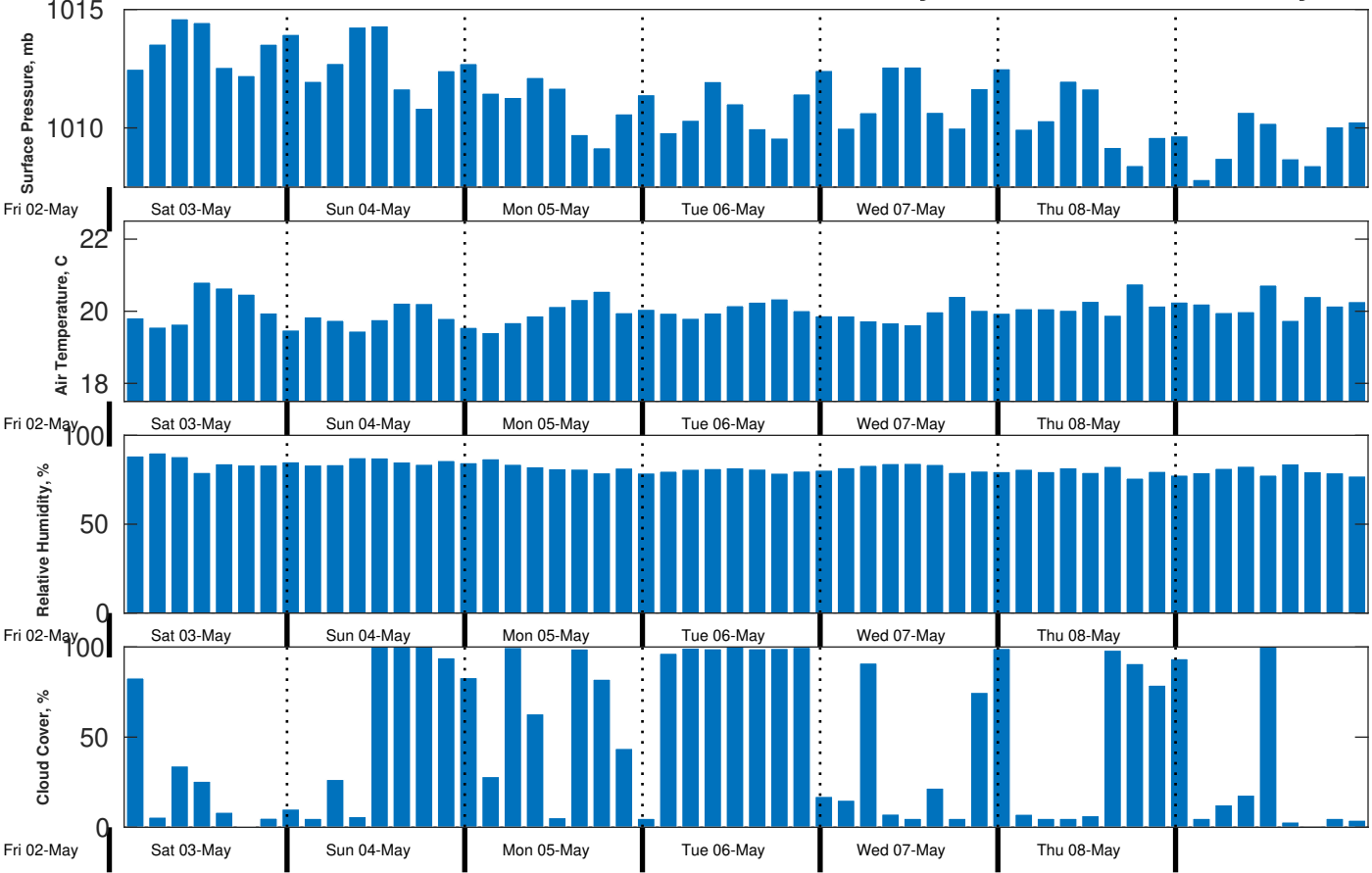
Met Forecast for CSA (ONHYM) PPL EBS - Mauritania from 03-May-2025 00:00:00 to 10-May-2025 00:00:00
