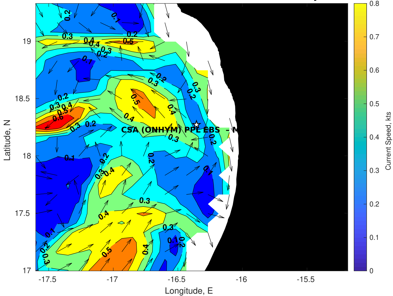
Surface Currents for CSA (ONHYM) PPL EBS - Mauritania at 02-May-2025 00:00:00
