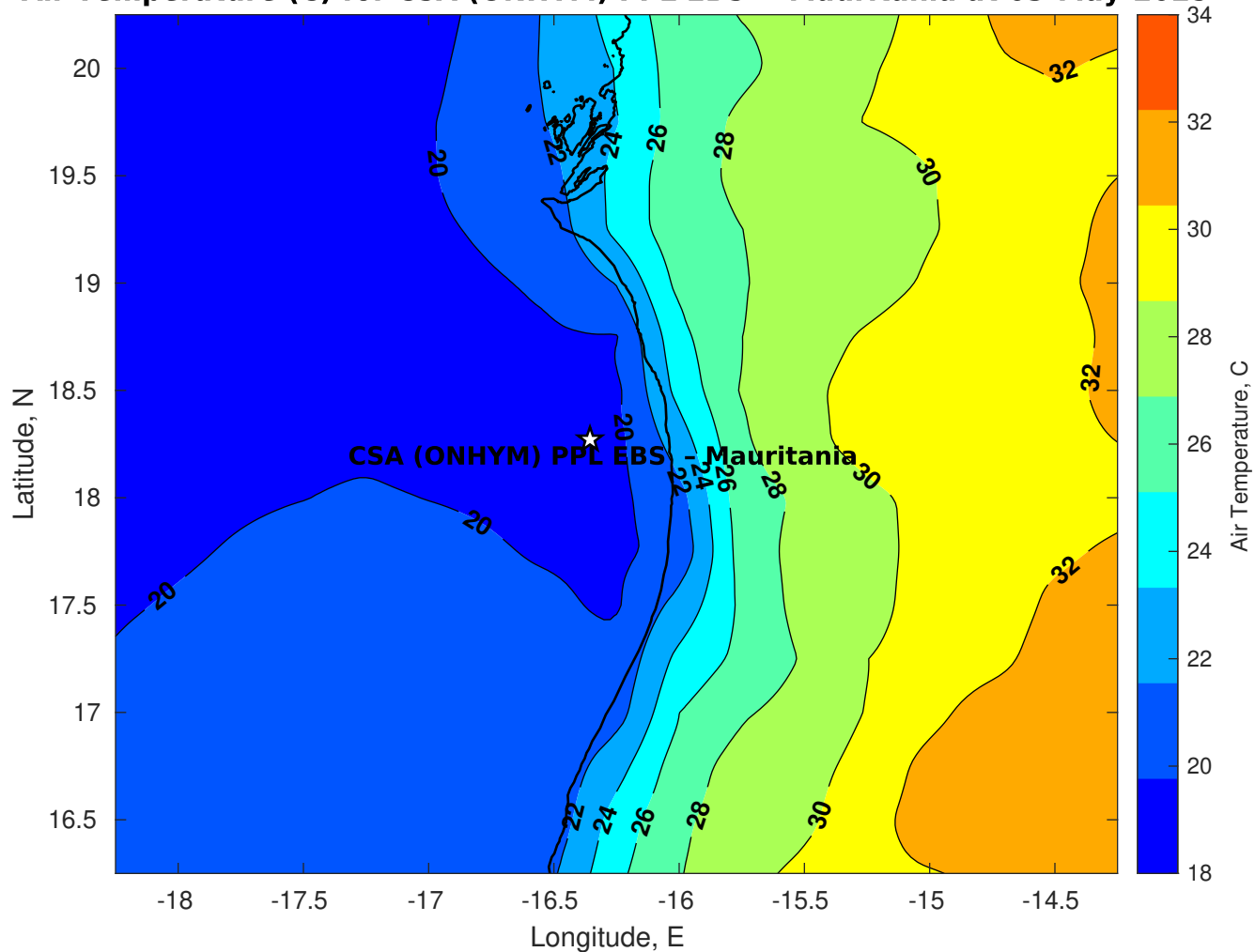
Air Temperature (C) for CSA (ONHYM) PPL EBS - Mauritania at 03-May-2025
