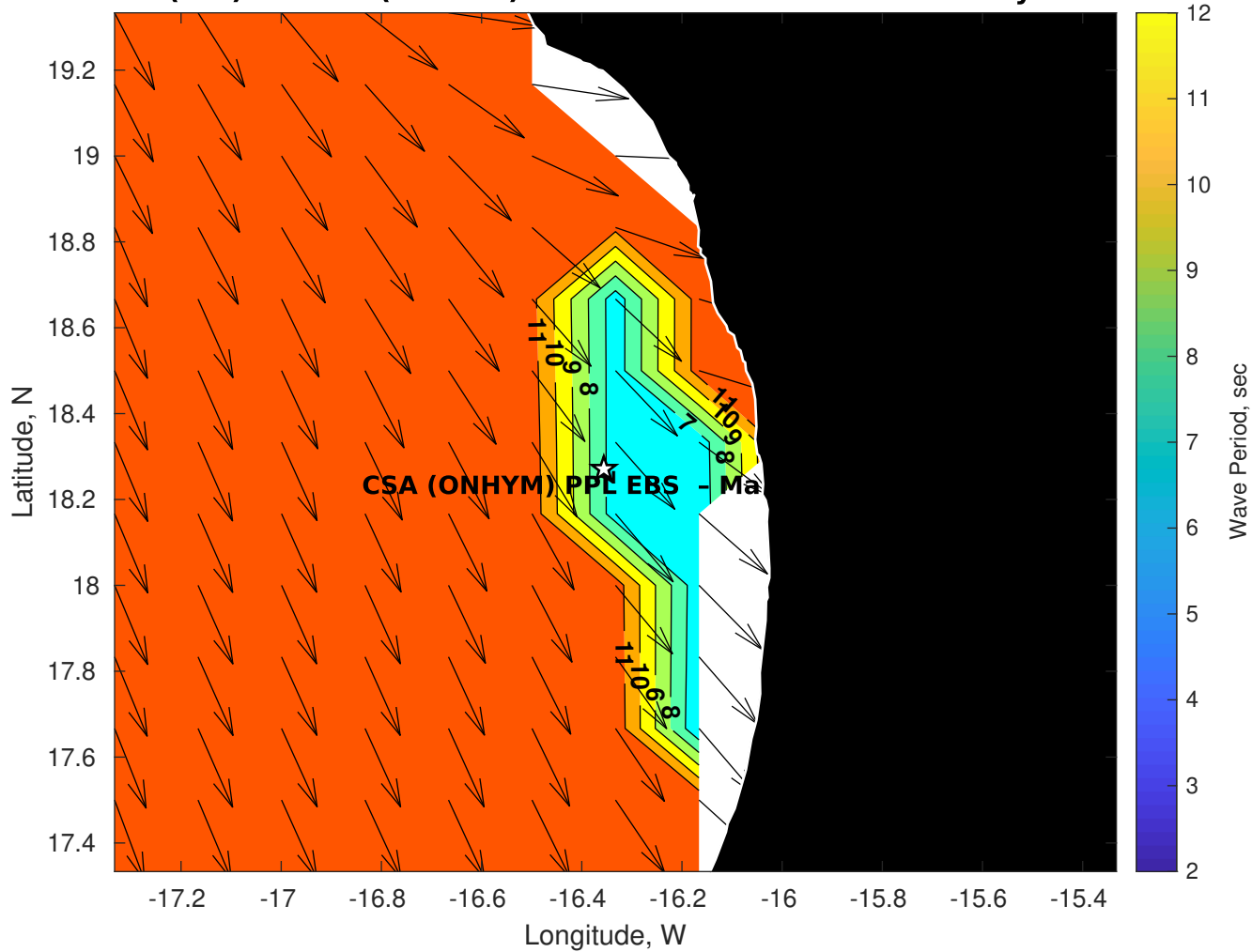
Wave Period (sec) for CSA (ONHYM) PPL EBS - Mauritania at 03-May-2025 09:00:00
