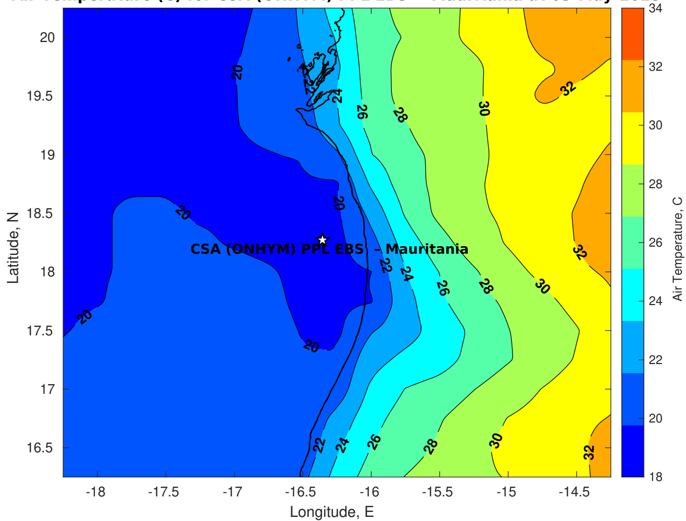
Air Temperature (C) for CSA (ONHYM) PPL EBS - Mauritania at 03-May-2025
