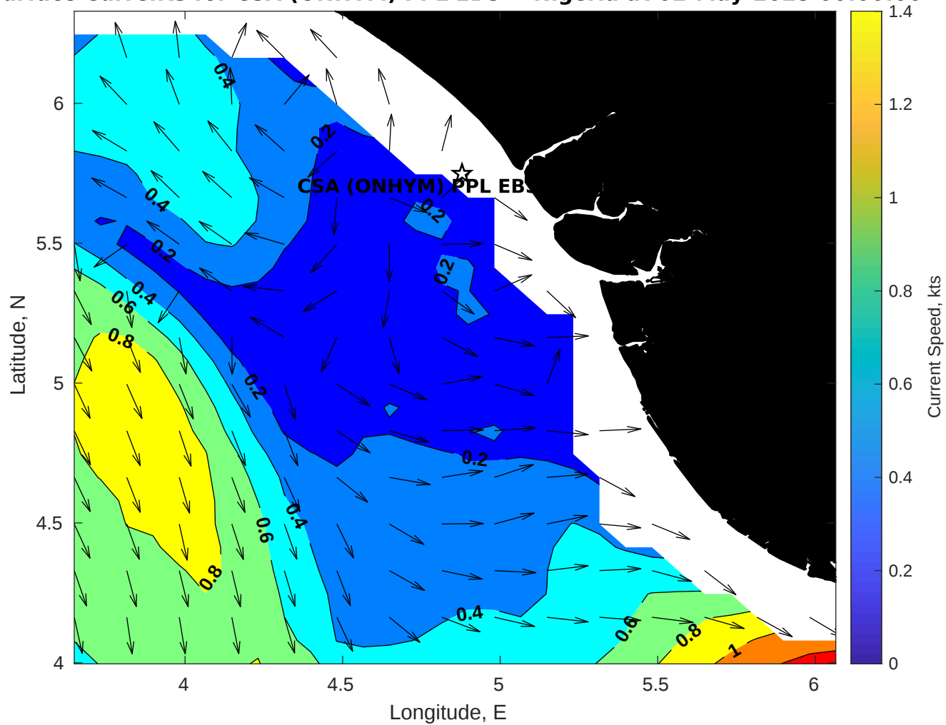
Surface Currents for CSA (ONHYM) PPL EBS - Nigeria at 02-May-2025 00:00:00
