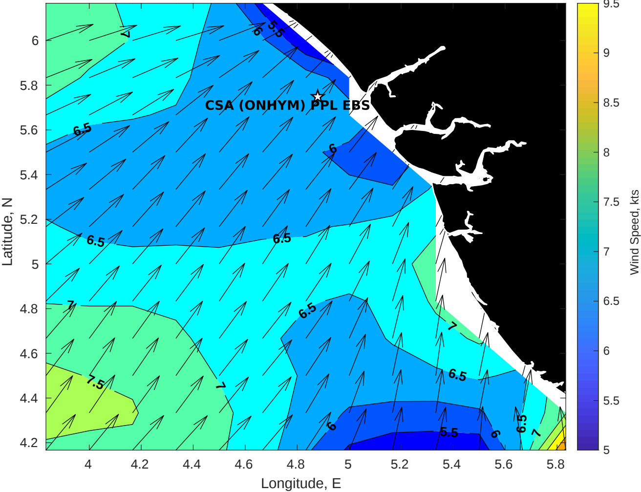
Winds (kts) for CSA (ONHYM) PPL EBS - Nigeria at 03-May-2025 09:00:00
