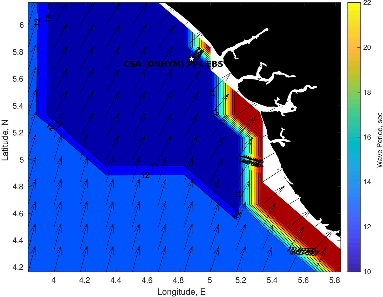
Wave Period (sec) for CSA (ONHYM) PPL EBS - Nigeria at 03-May-2025 09:00:00
