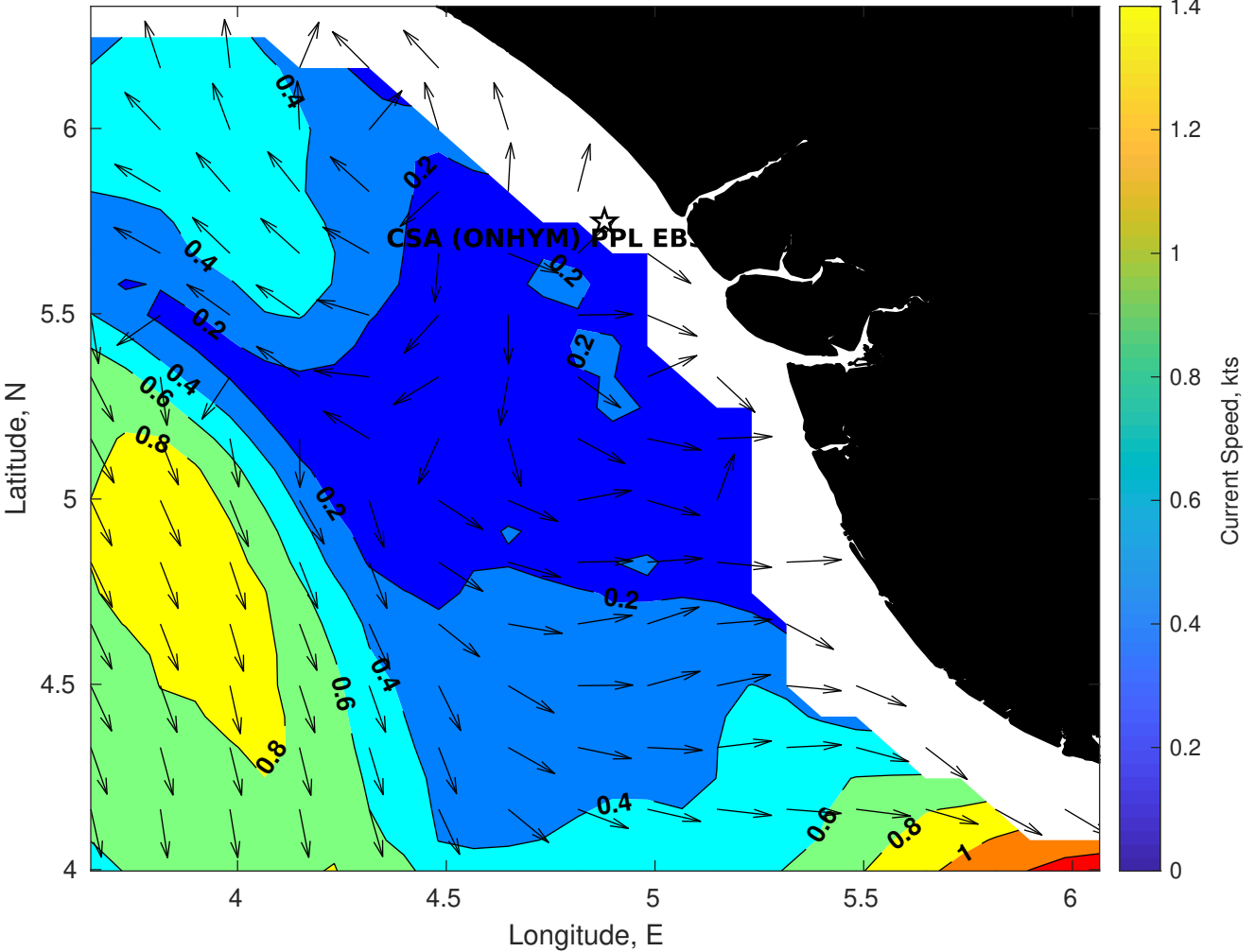
Surface Currents for CSA (ONHYM) PPL EBS - Nigeria at 02-May-2025 00:00:00
