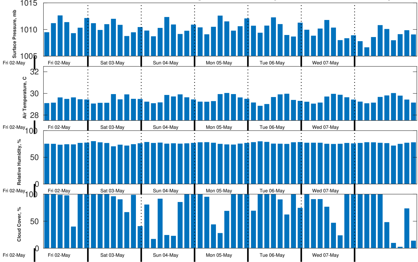
Met Forecast for CSA (ONHYM) PPL EBS - Nigeria from 03-May-2025 00:00:00 to 10-May-2025 00:00:00
