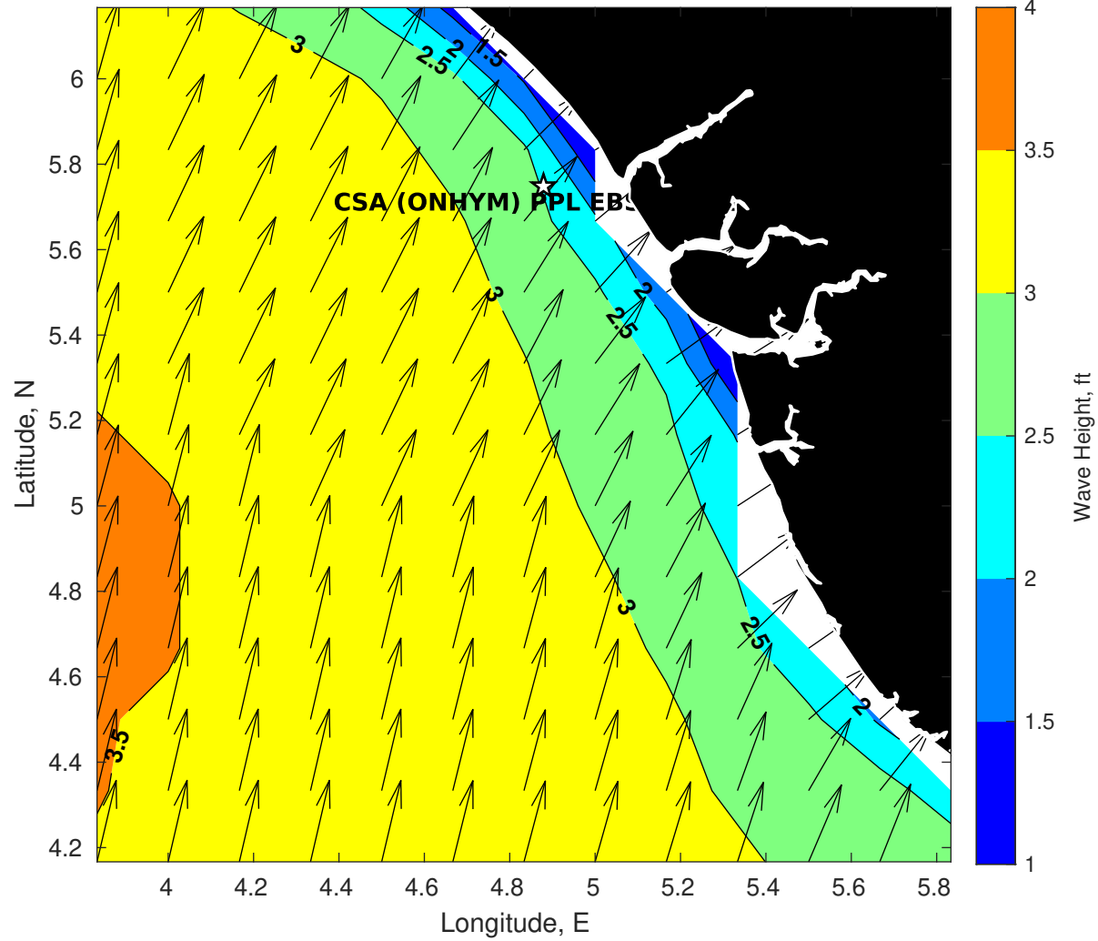
Wave Height (ft) for CSA (ONHYM) PPL EBS - Nigeria at 03-May-2025 09:00:00
