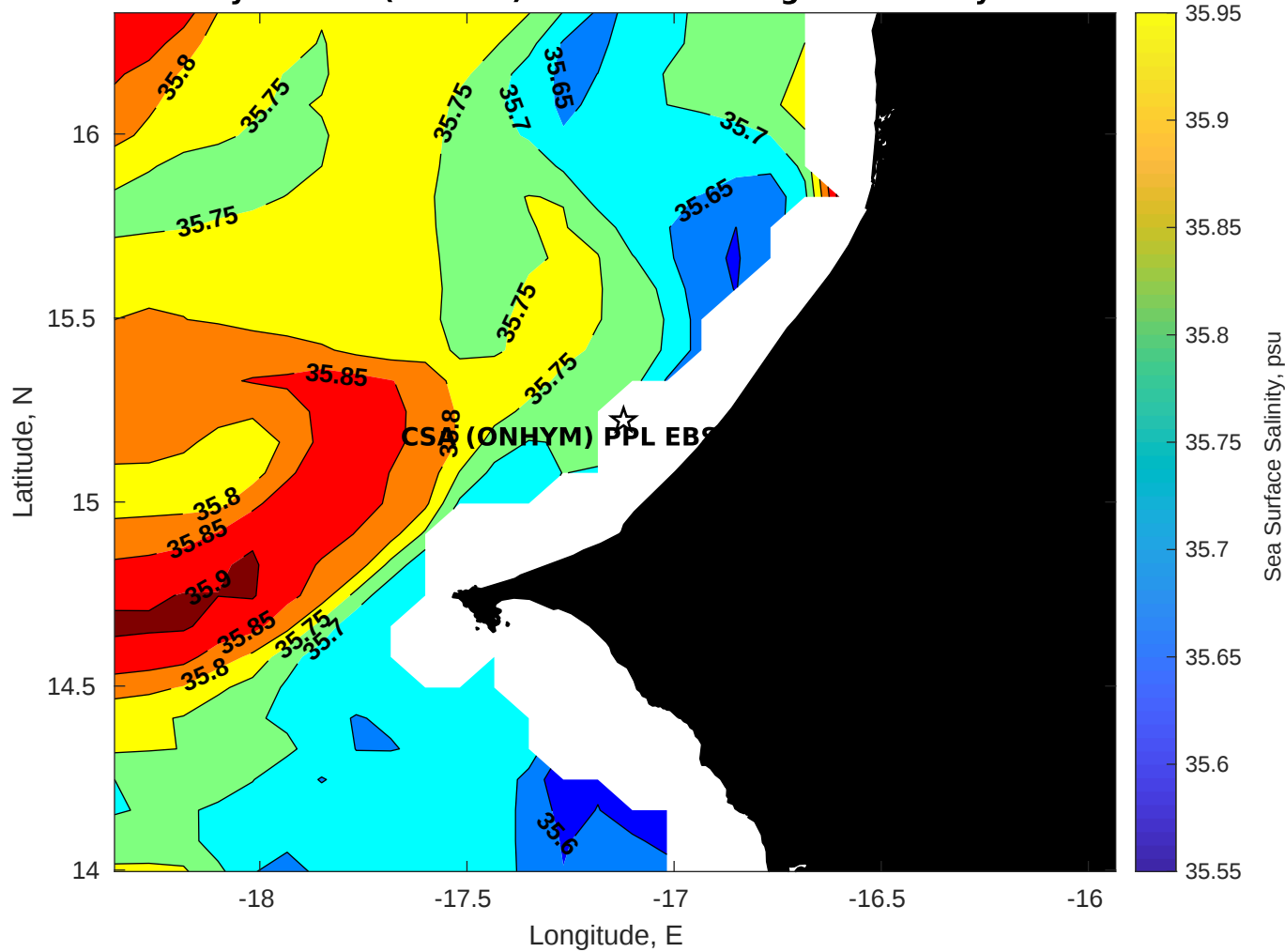
Surface Salinity for CSA (ONHYM) PPL EBS - Senegal at 02-May-2025 00:00:00
