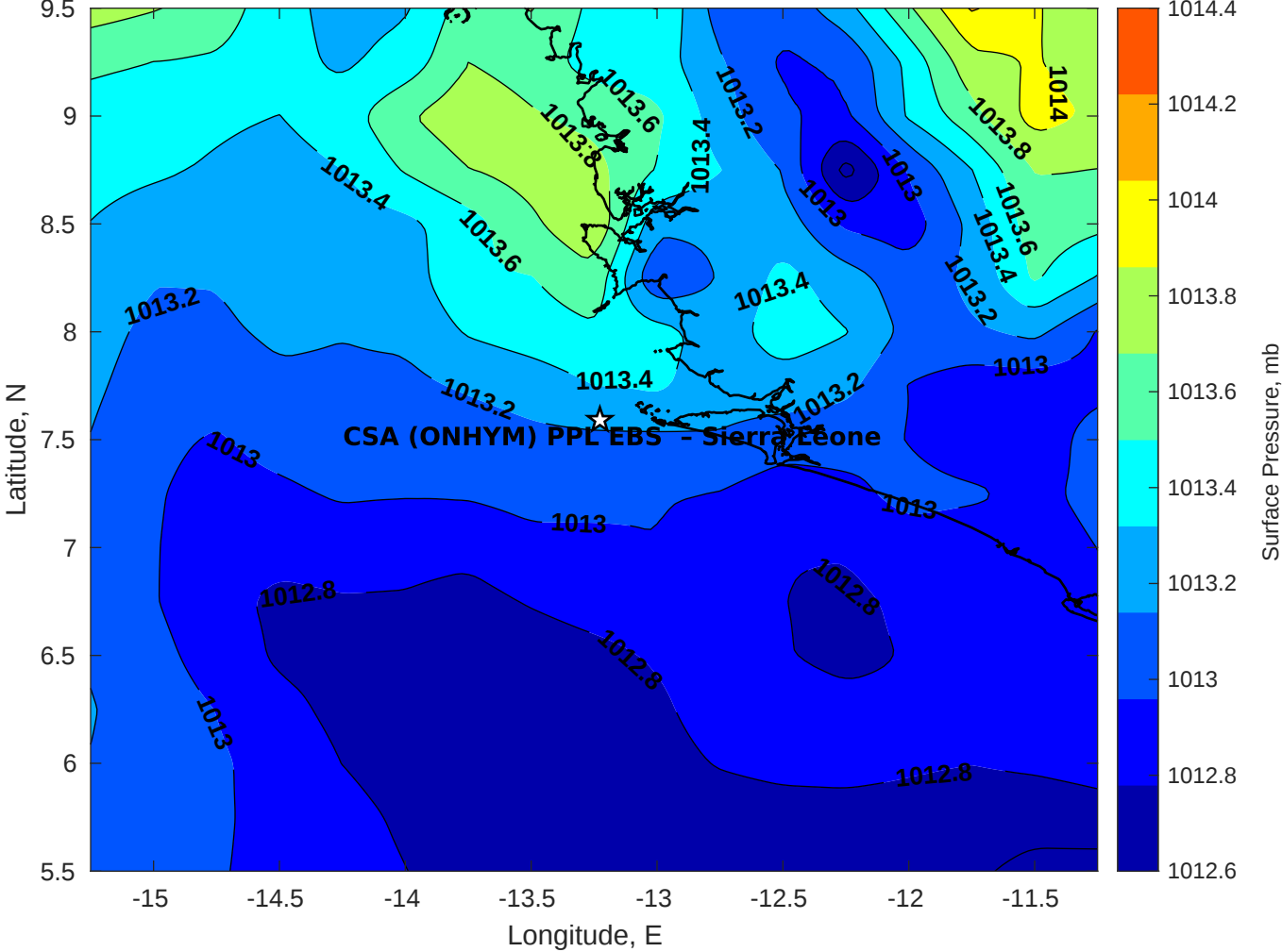
Surface Pressure (mb) for CSA (ONHYM) PPL EBS - Sierra Leone at 04-May-2025 00:00:00
