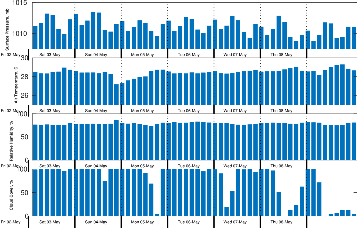
Met Forecast for CSA (ONHYM) PPL EBS - Sierra Leone from 03-May-2025 00:00:00 to 10-May-2025 00:00:00
