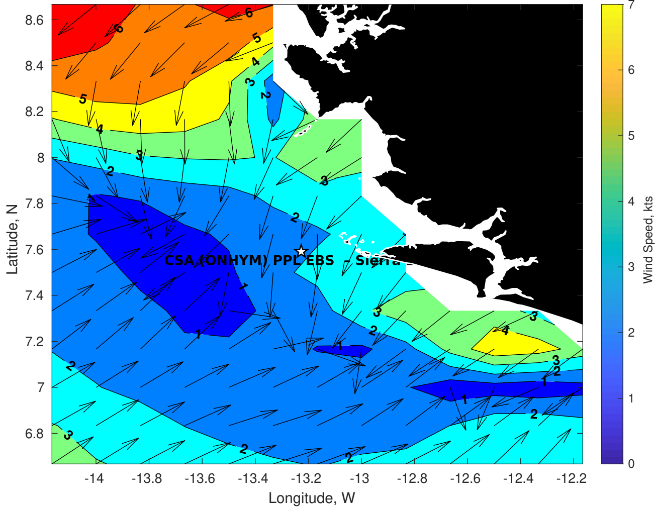
Winds (kts) for CSA (ONHYM) PPL EBS - Sierra Leone at 03-May-2025 09:00:00
