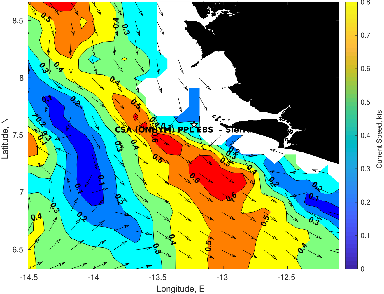
Surface Currents for CSA (ONHYM) PPL EBS - Sierra Leone at 02-May-2025 00:00:00
