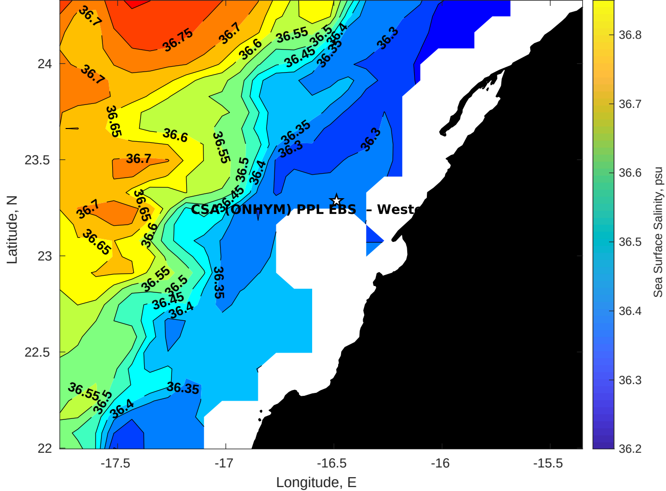
Surface Salinity for CSA (ONHYM) PPL EBS - Western Sahara at 02-May-2025 00:00:00
