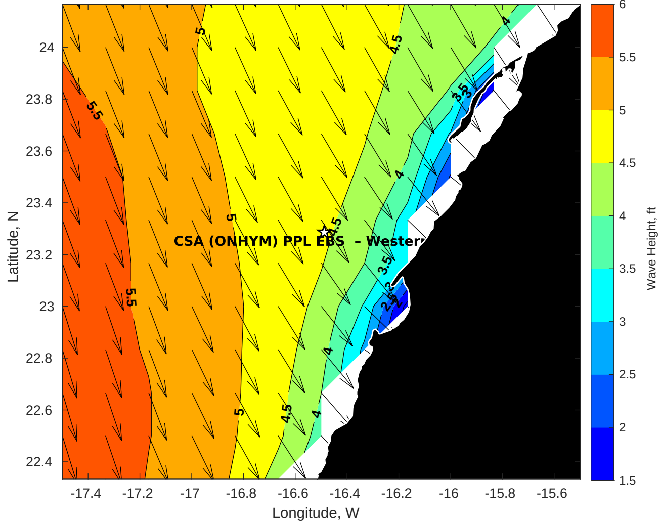
Wave Height (ft) for CSA (ONHYM) PPL EBS - Western Sahara at 03-May-2025 09:00:00
