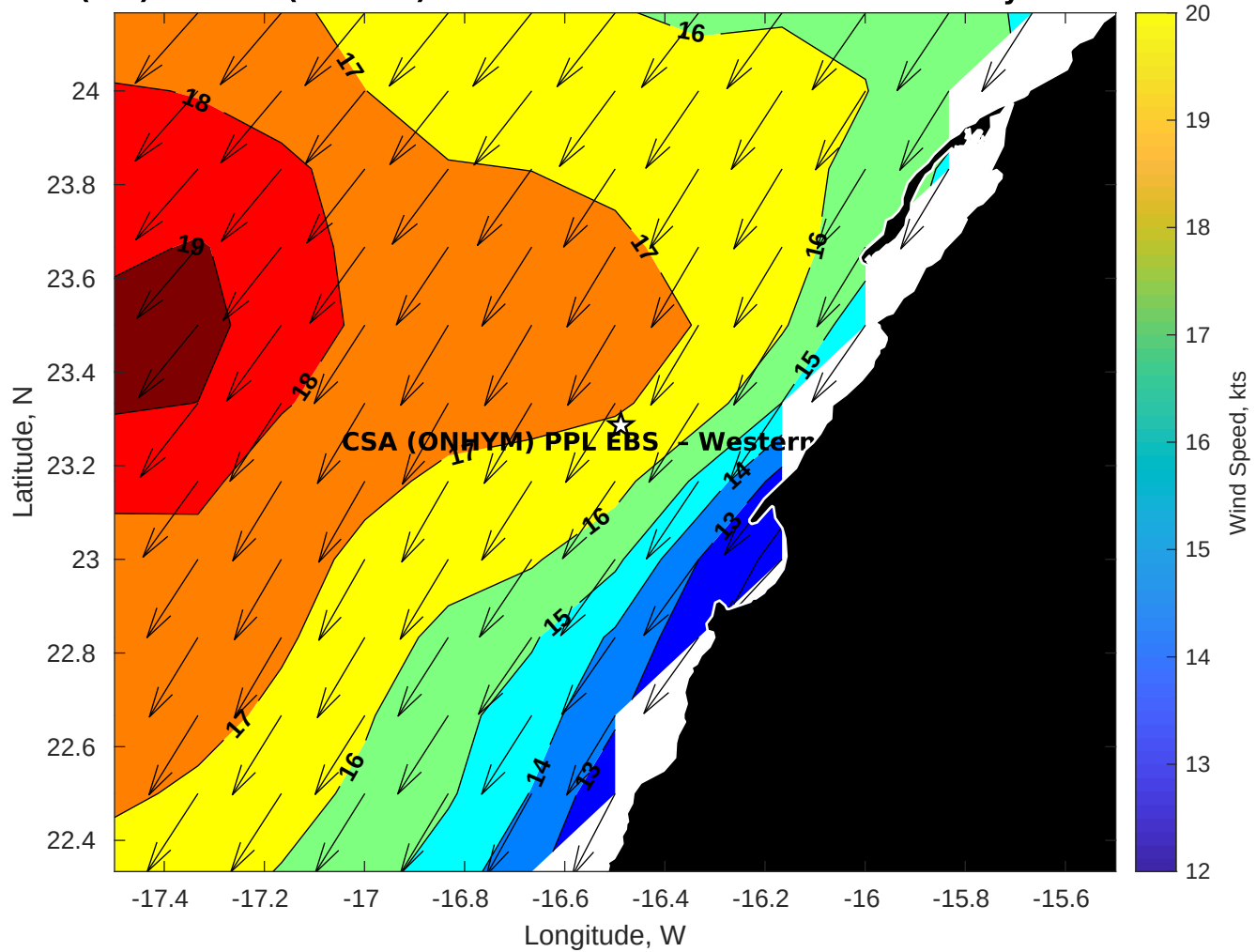
Winds (kts) for CSA (ONHYM) PPL EBS - Western Sahara at 03-May-2025 09:00:00
