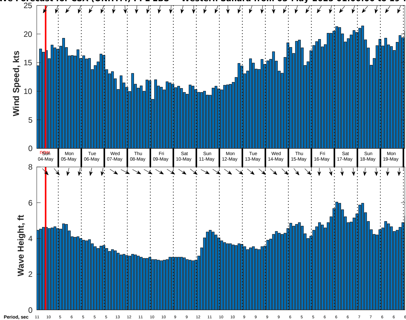
Wind & Wave Forecast for CSA (ONHYM) PPL EBS - Western Sahara from 03-May-2025 01:00:00 to 19-May-2025 01:00:00
