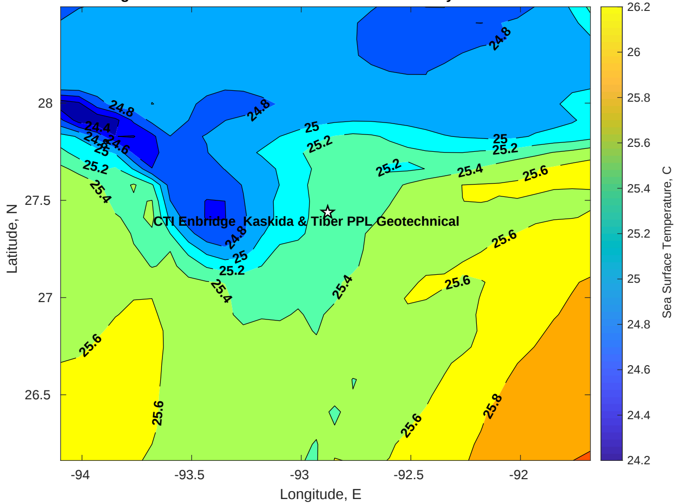
SST for CTI Enbridge Kaskida & Tiber PPL Geotechnical at 02-May-2025 00:00:00
