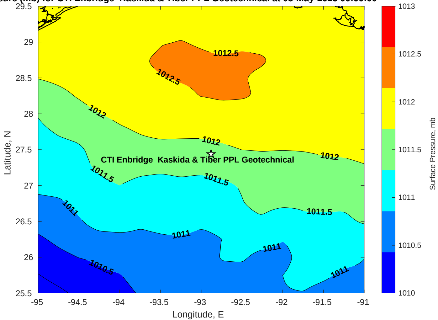
Surface Pressure (mb) for CTI Enbridge Kaskida & Tiber PPL Geotechnical at 05-May-2025 00:00:00
