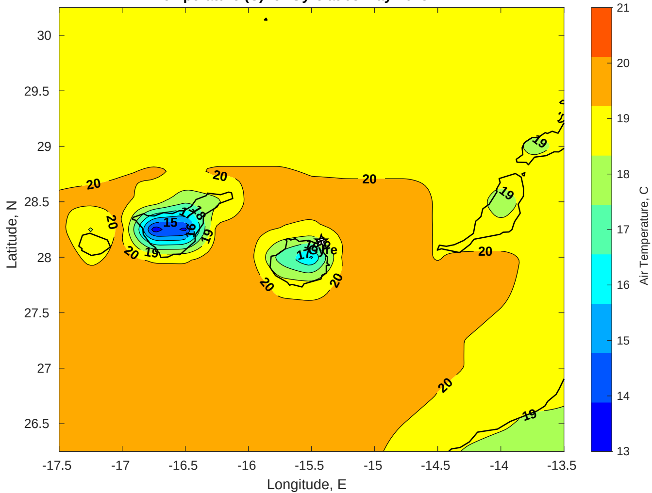
Air Temperature (C) for Gyre at 03-May-2025
