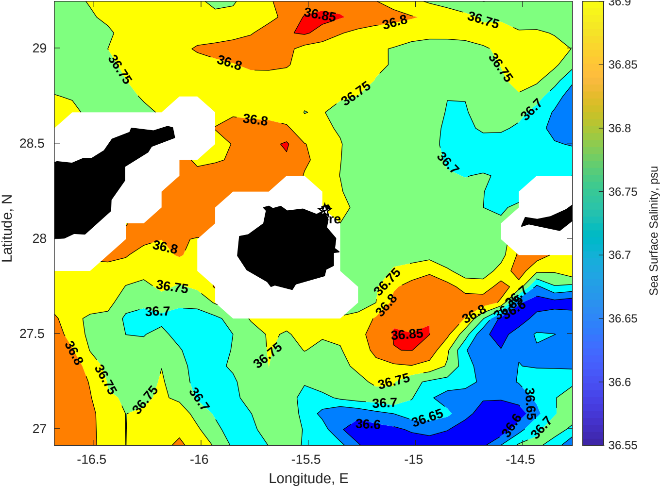
Surface Salinity for Gyre at 02-May-2025 00:00:00
