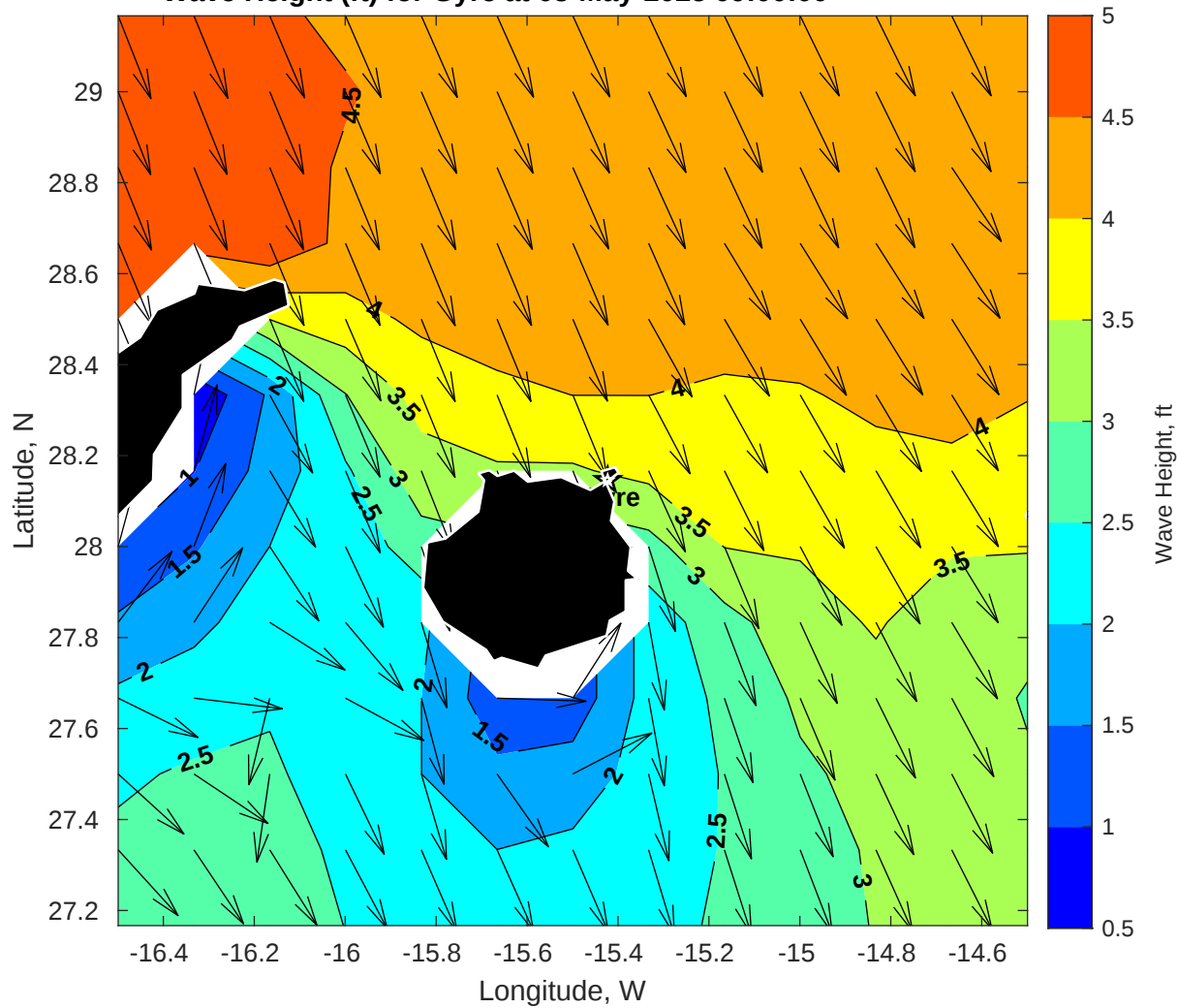
Wave Height (ft) for Gyre at 03-May-2025 09:00:00
