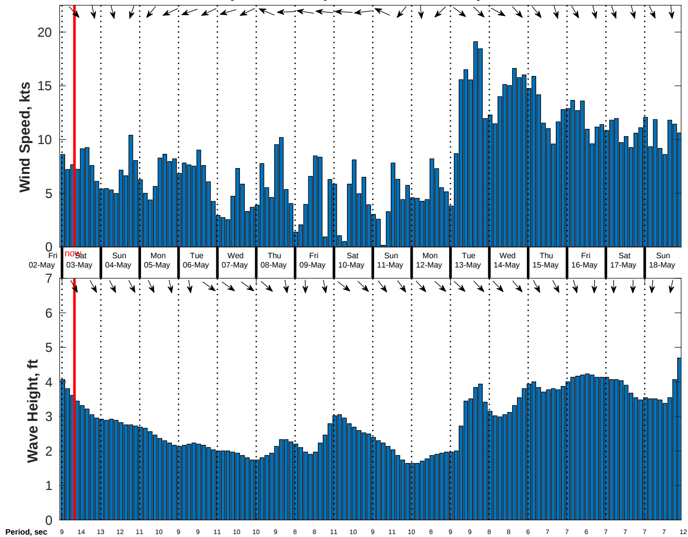
Wind & Wave Forecast for Gyre from 02-May-2025 23:00:00 to 18-May-2025 23:00:00
