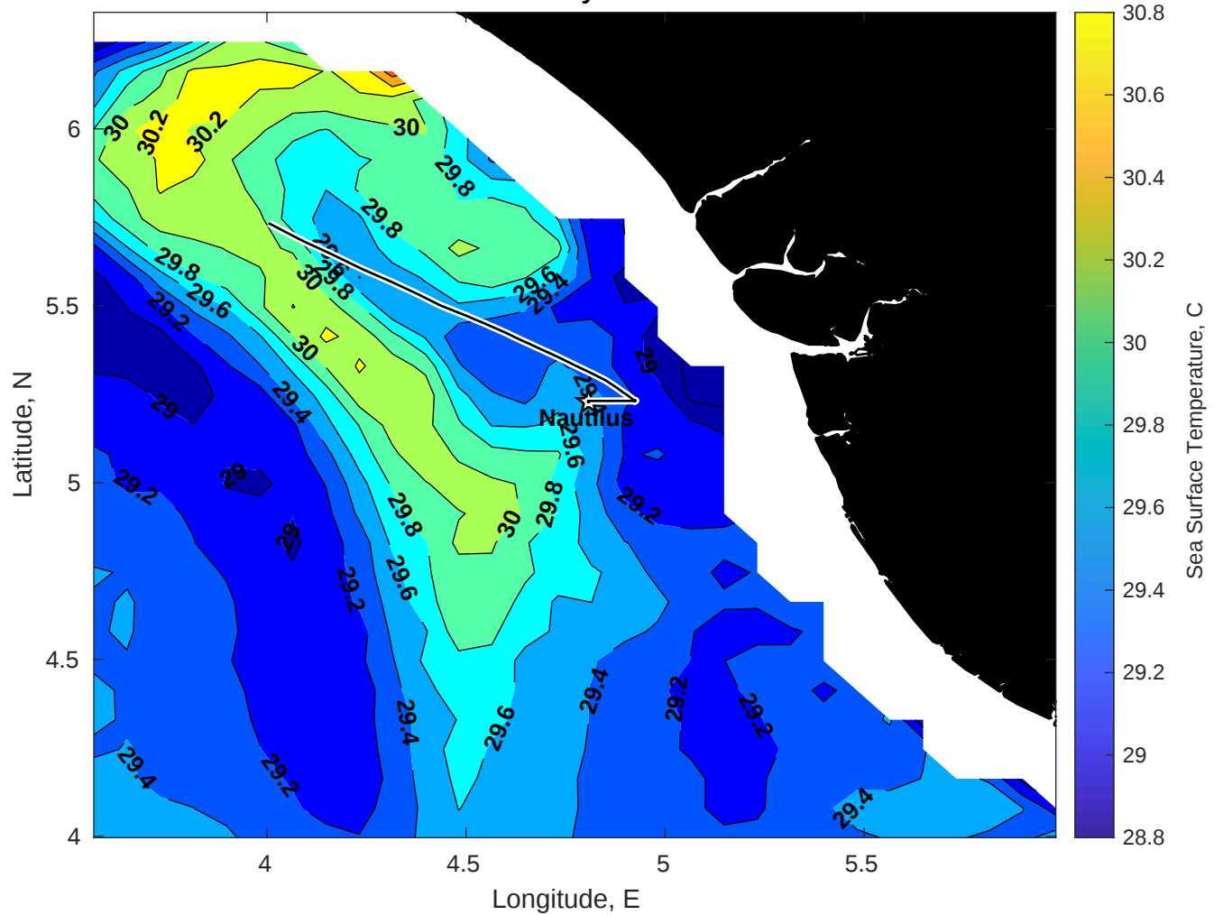
SST for Nautilus at 02-May-2025 00:00:00
