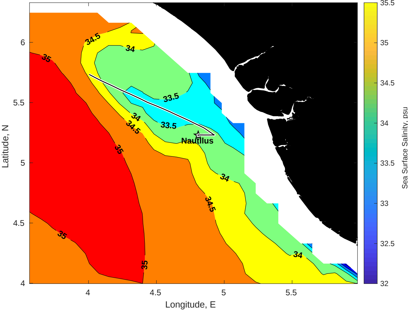
Surface Salinity for Nautilus at 02-May-2025 00:00:00
