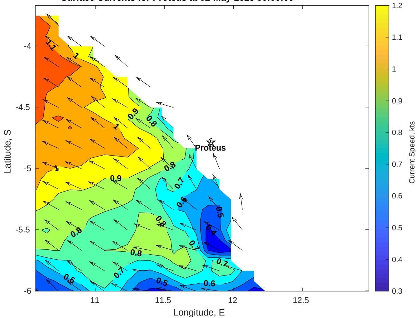
Surface Currents for Proteus at 02-May-2025 00:00:00
