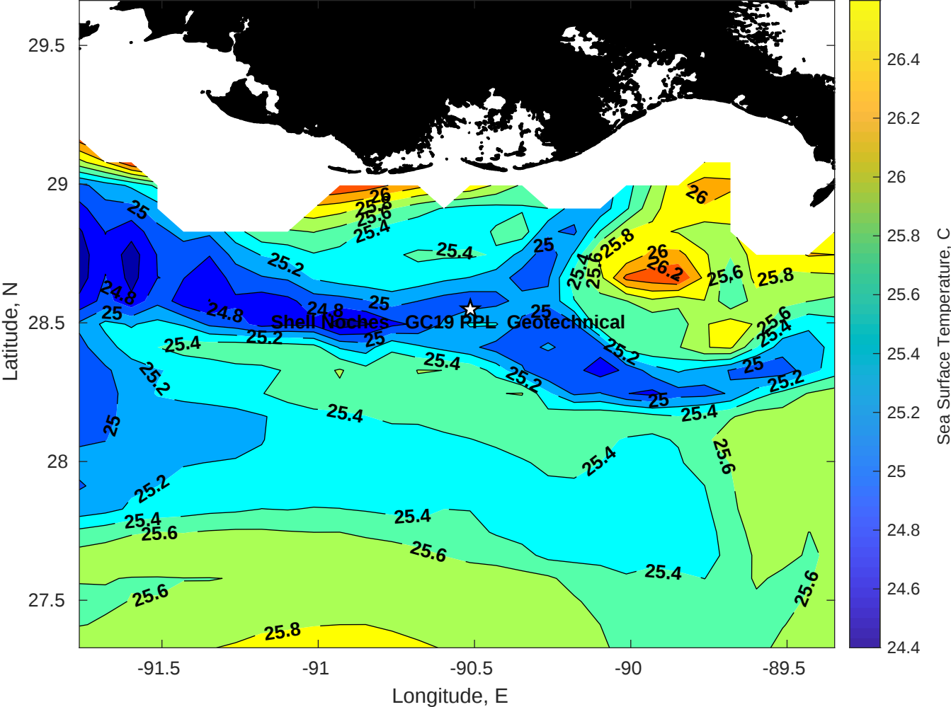
SST for Shell Noches GC19 PPL Geotechnical at 02-May-2025 00:00:00
