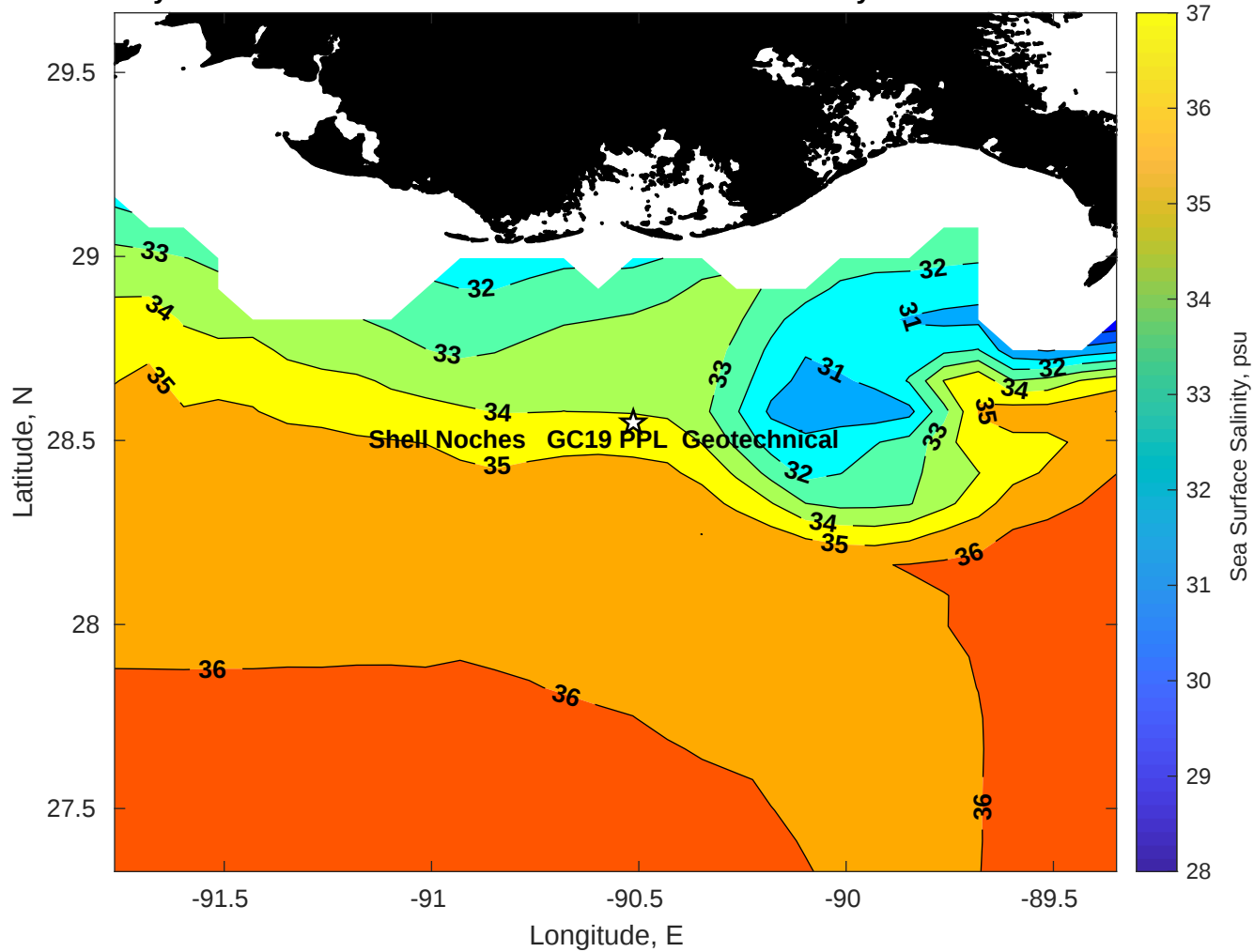
Surface Salinity for Shell Noches GC19 PPL Geotechnical at 02-May-2025 00:00:00
