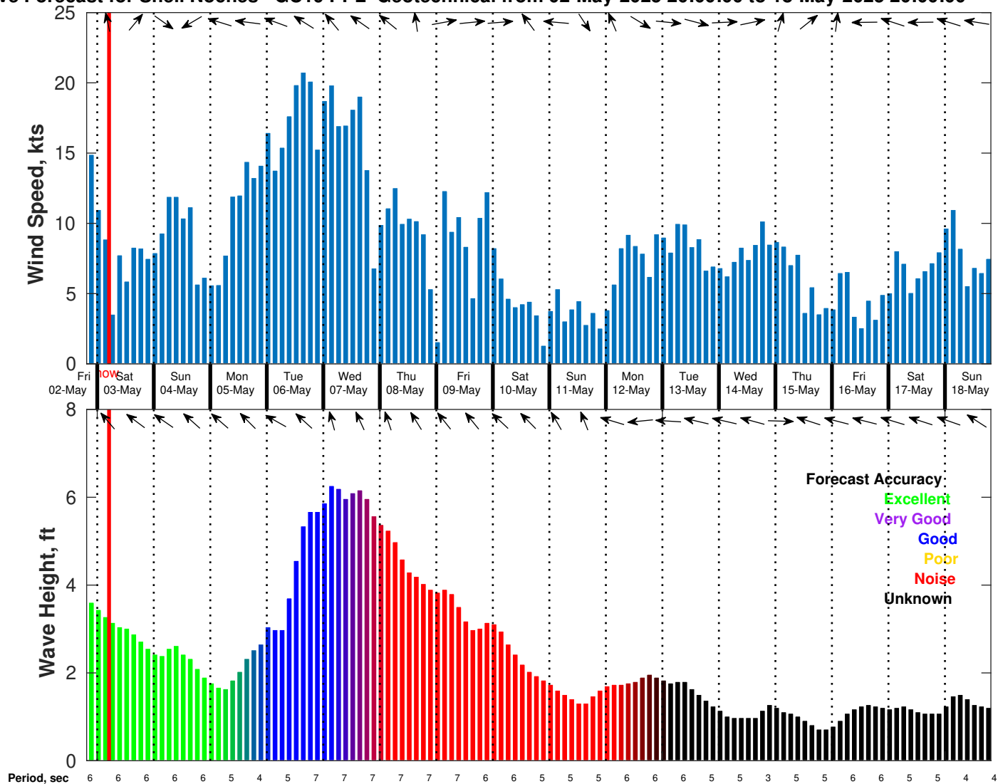
Wind & Wave Forecast for Shell Noches GC19 PPL Geotechnical from 02-May-2025 20:00:00 to 18-May-2025 20:00:00
