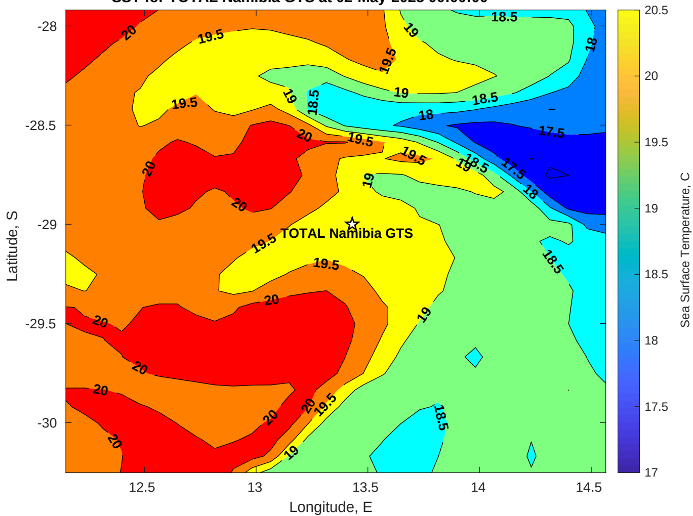
SST for TOTAL Namibia GTS at 02-May-2025 00:00:00
