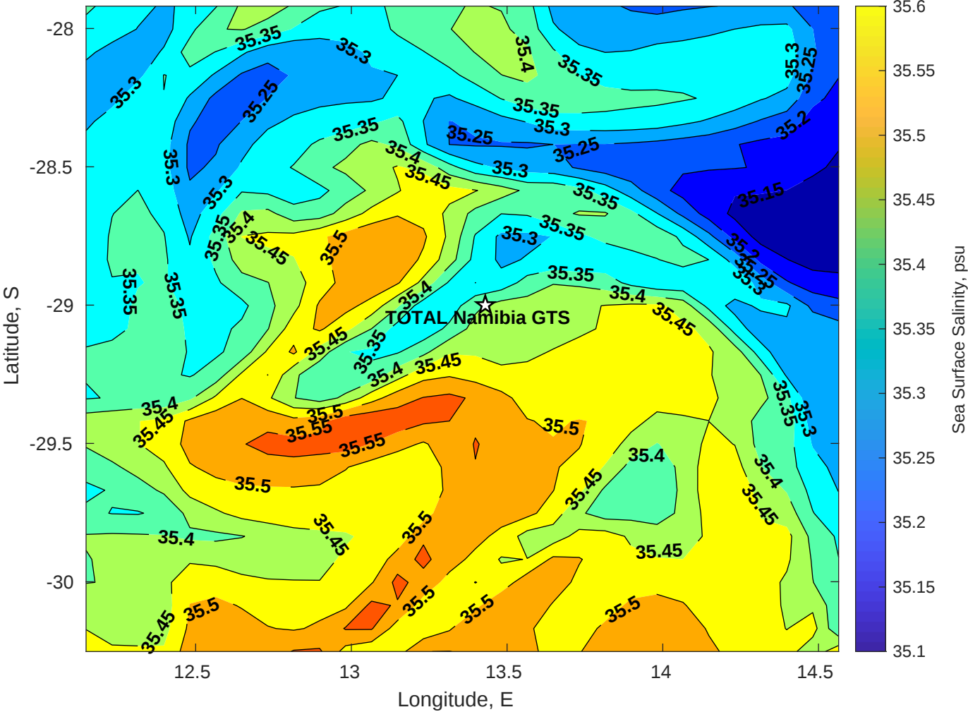
Surface Salinity for TOTAL Namibia GTS at 02-May-2025 00:00:00
