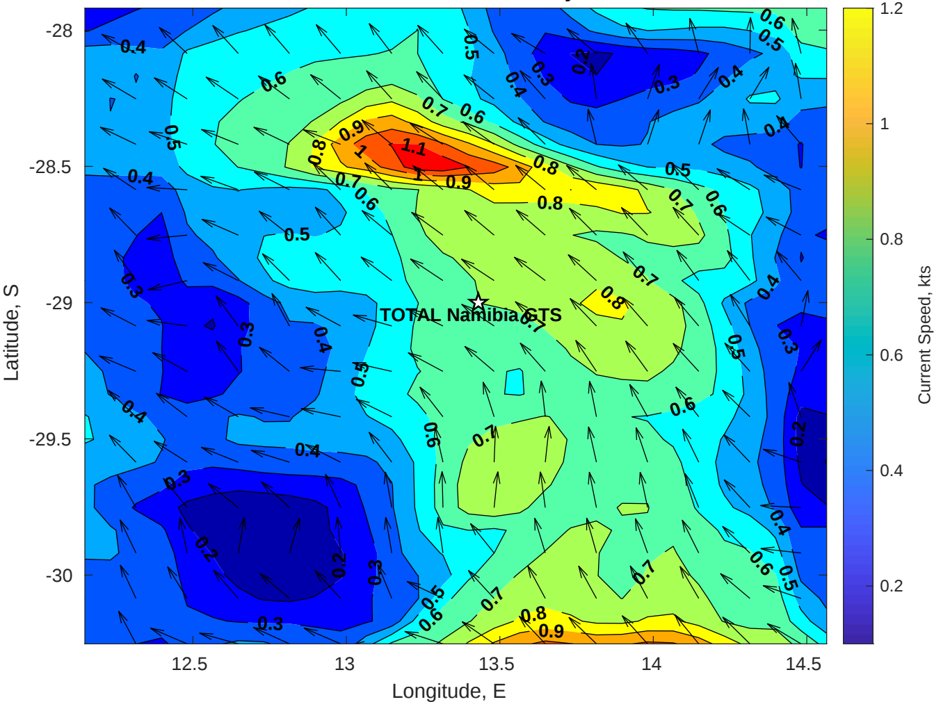
Surface Currents for TOTAL Namibia GTS at 02-May-2025 00:00:00
