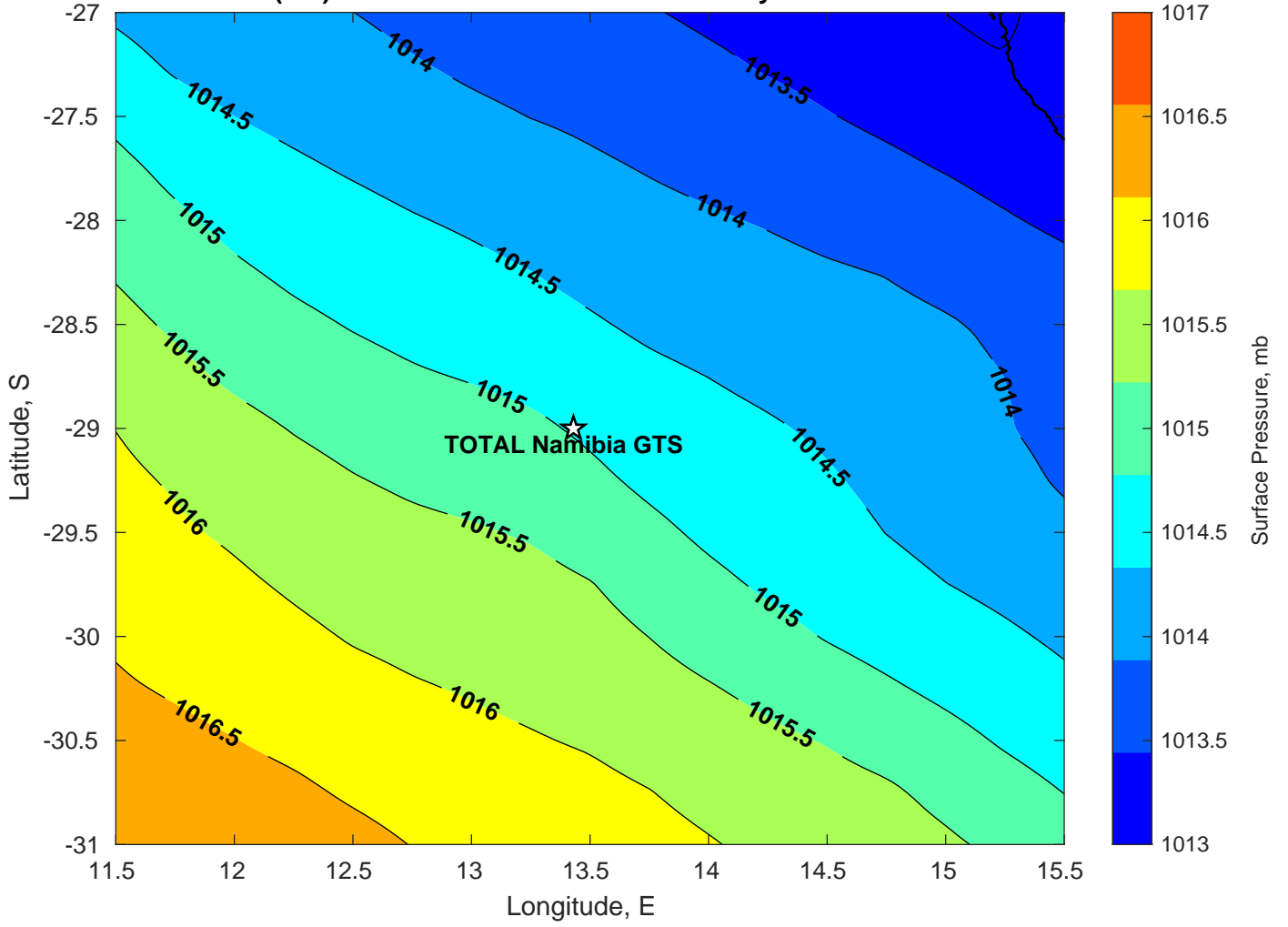
Surface Pressure (mb) for TOTAL Namibia GTS at 05-May-2025 00:00:00
