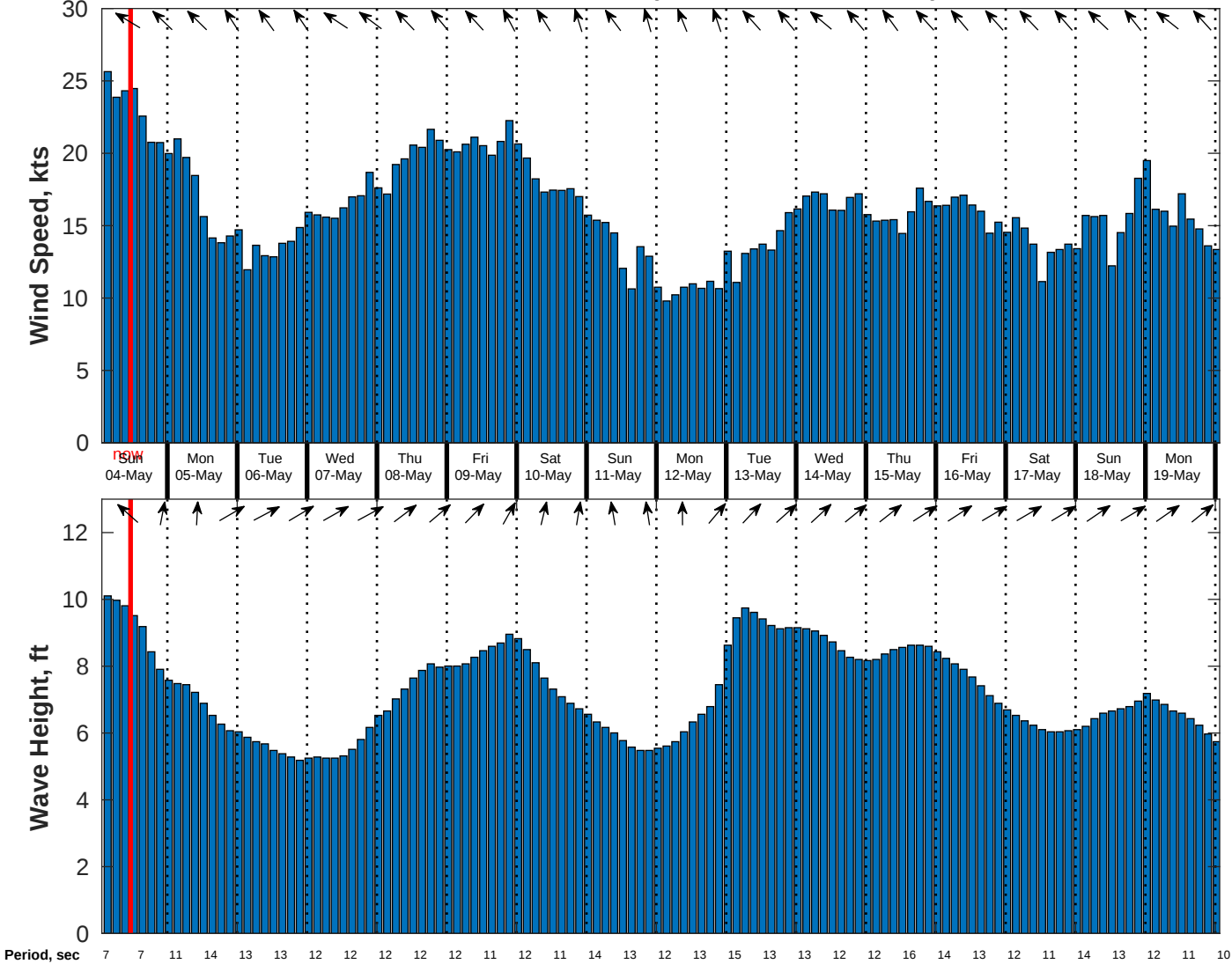
Wind & Wave Forecast for TOTAL Namibia GTS from 03-May-2025 02:00:00 to 19-May-2025 02:00:00
