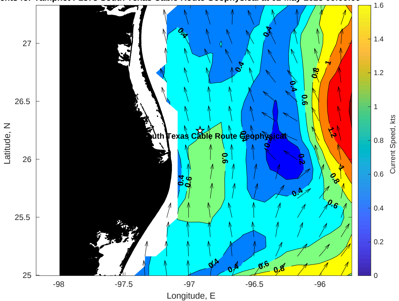
Surface Currents for Tampnet P2378 South Texas Cable Route Geophysical at 02-May-2025 00:00:00
