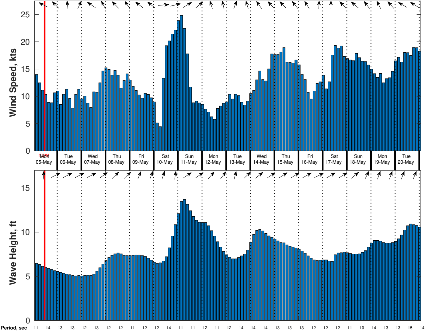
Wind & Wave Forecast for Benthic Solutions South Africa HF Site1 from 04-May-2025 02:00:00 to 20-May-2025 02:00:00
