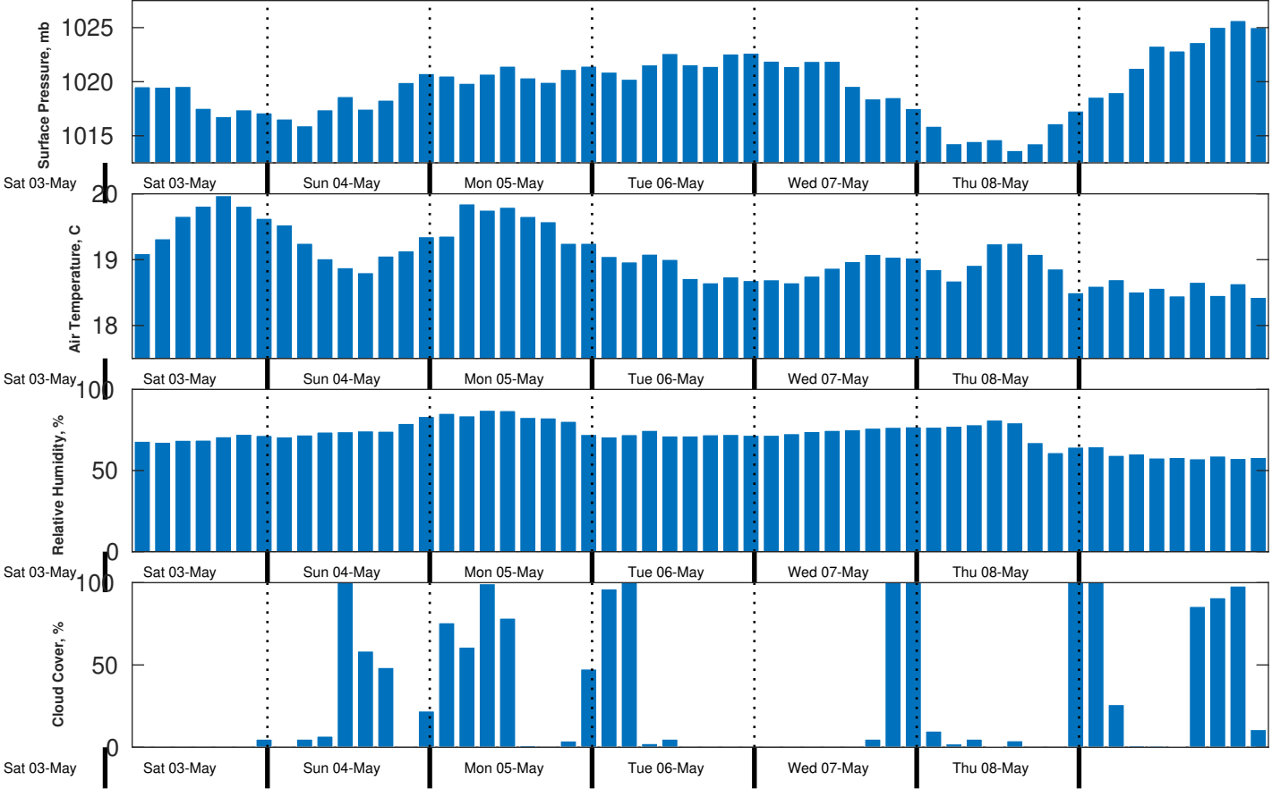
Met Forecast for Benthic Solutions South Africa HF Site1 from 04-May-2025 00:00:00 to 11-May-2025 00:00:00
