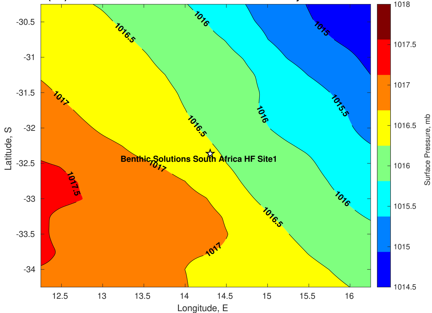
Surface Pressure (mb) for Benthic Solutions South Africa HF Site1 at 05-May-2025 00:00:00
