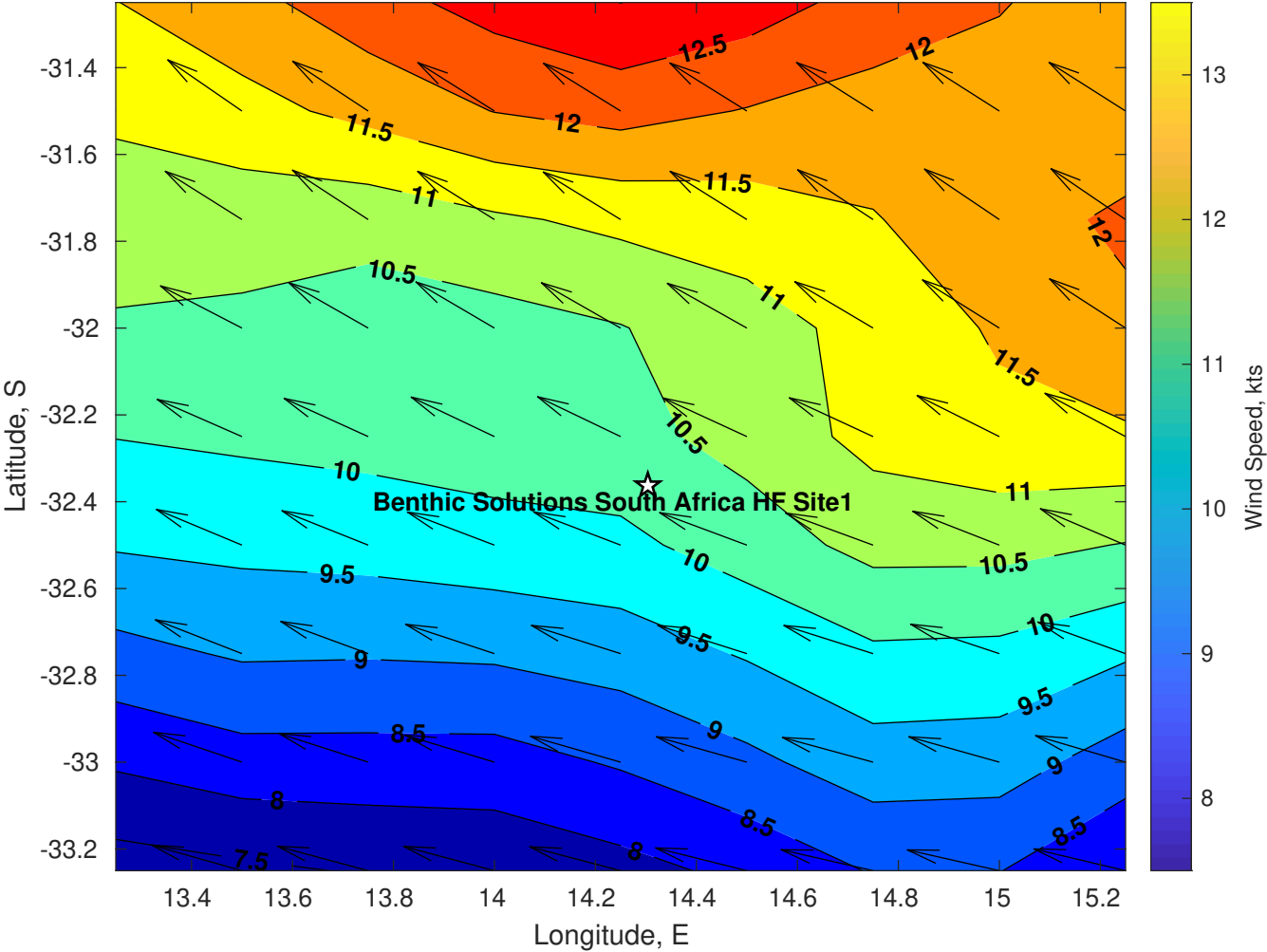
Winds (kts) for Benthic Solutions South Africa HF Site1 at 04-May-2025 09:00:00
