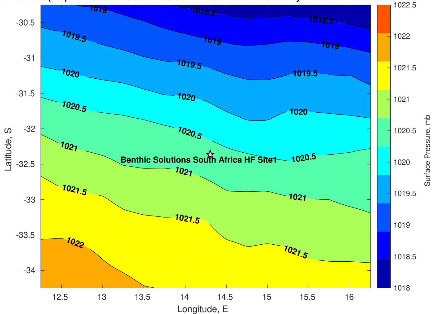
Surface Pressure (mb) for Benthic Solutions South Africa HF Site1 at 04-May-2025 00:00:00
