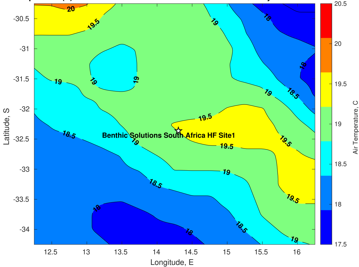
Air Temperature (C) for Benthic Solutions South Africa HF Site1 at 04-May-2025
