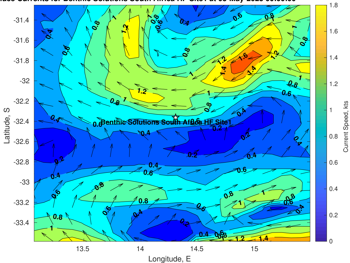
Surface Currents for Benthic Solutions South Africa HF Site1 at 03-May-2025 00:00:00
