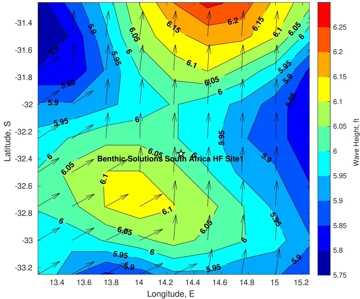
Wave Height (ft) for Benthic Solutions South Africa HF Site1 at 04-May-2025 09:00:00
