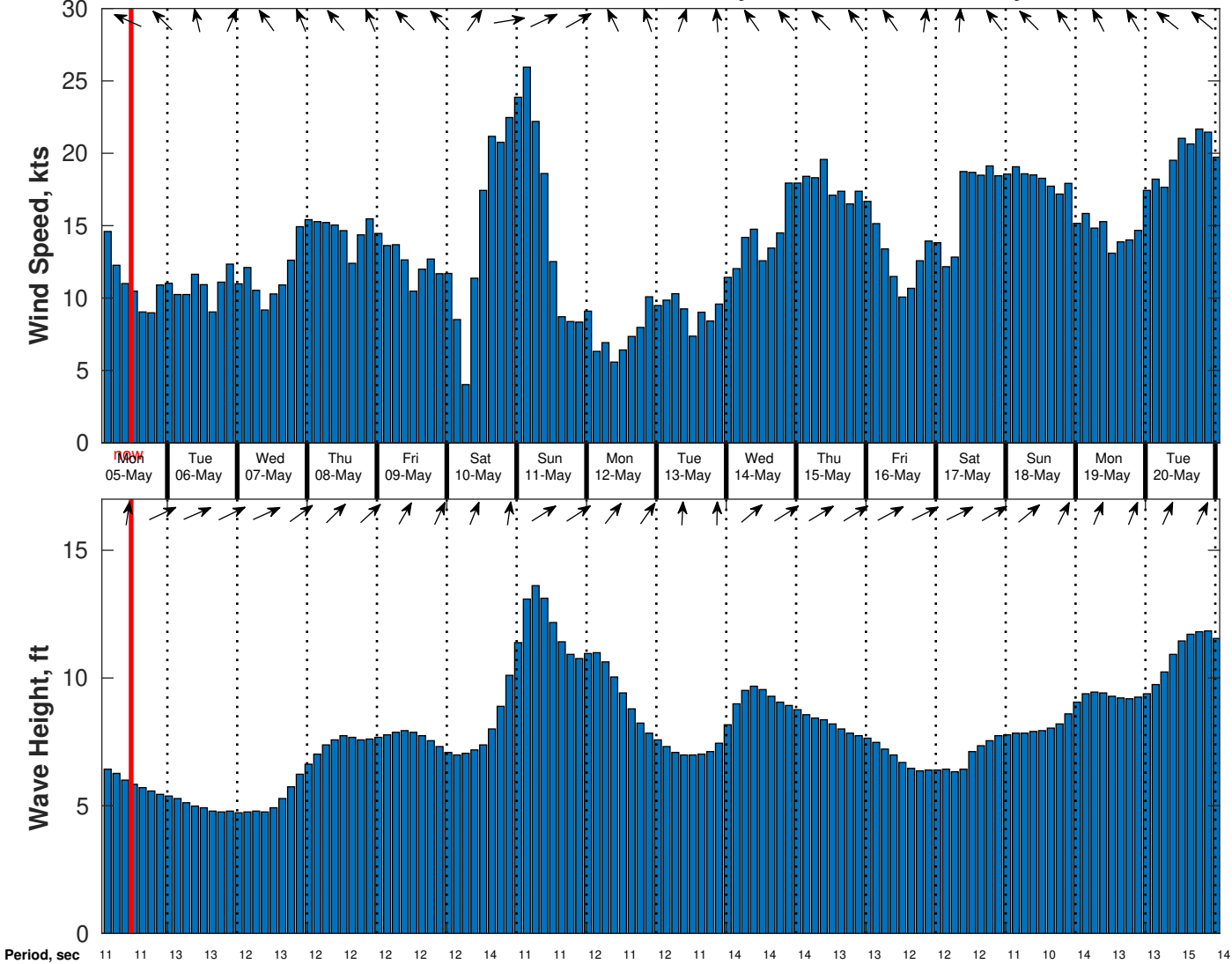
Wind & Wave Forecast for Benthic Solutions South Africa HF Site2 from 04-May-2025 02:00:00 to 20-May-2025 02:00:00
