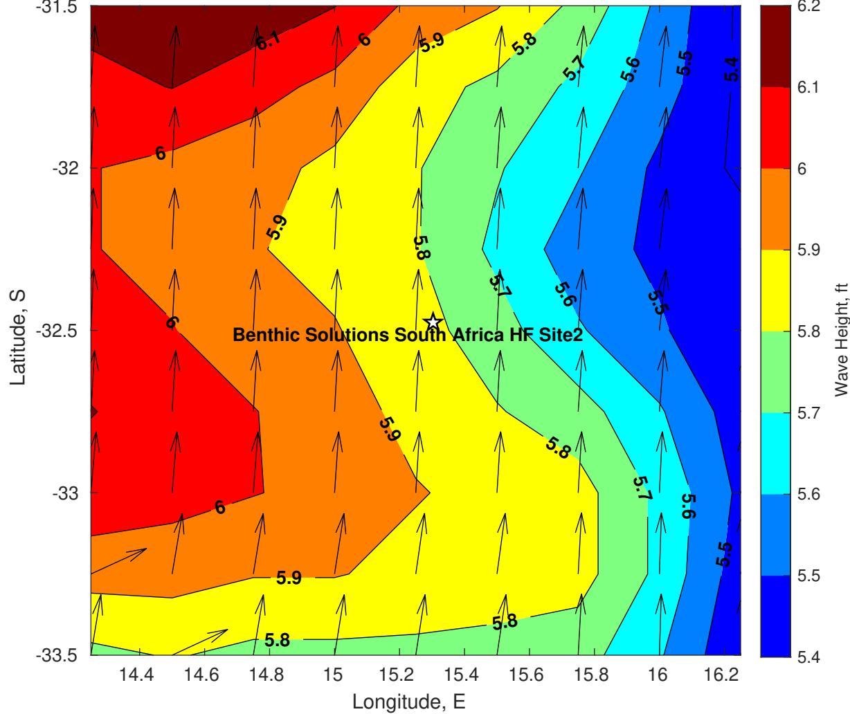
Wave Height (ft) for Benthic Solutions South Africa HF Site2 at 04-May-2025 09:00:00
