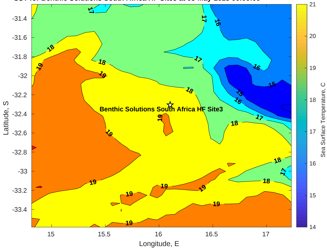
SST for Benthic Solutions South Africa HF Site3 at 03-May-2025 00:00:00
