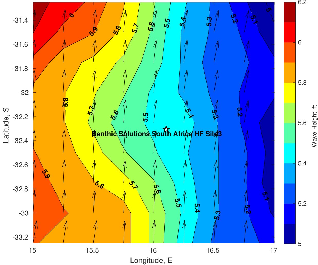
Wave Height (ft) for Benthic Solutions South Africa HF Site3 at 04-May-2025 09:00:00
