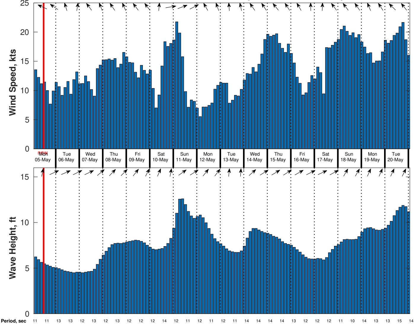
Wind & Wave Forecast for Benthic Solutions South Africa HF Site3 from 04-May-2025 02:00:00 to 20-May-2025 02:00:00
