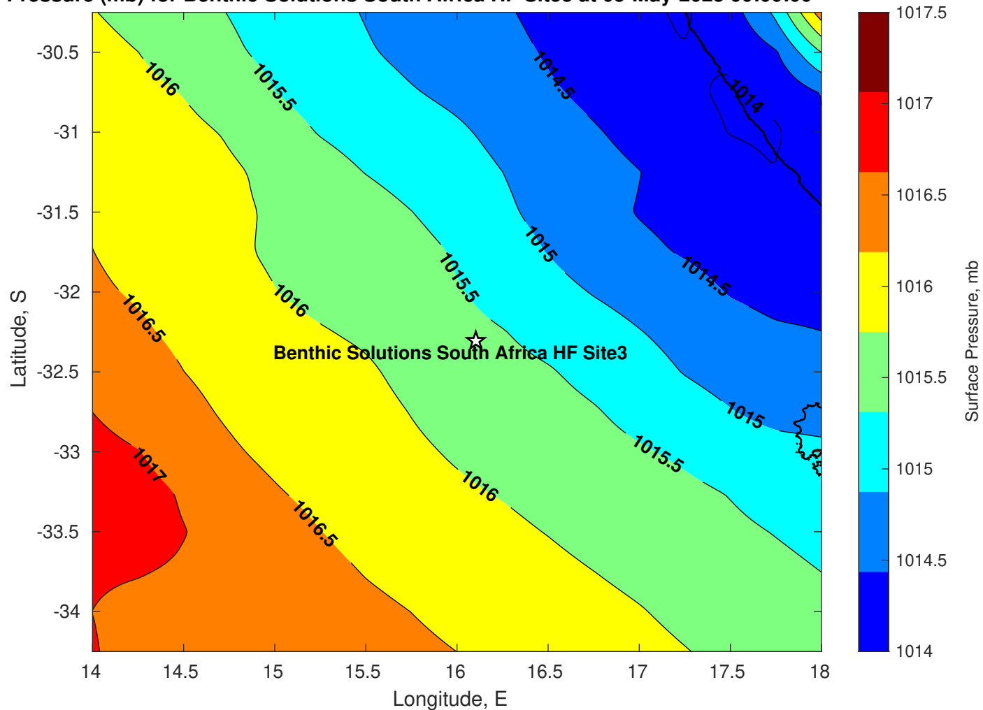
Surface Pressure (mb) for Benthic Solutions South Africa HF Site3 at 05-May-2025 00:00:00
