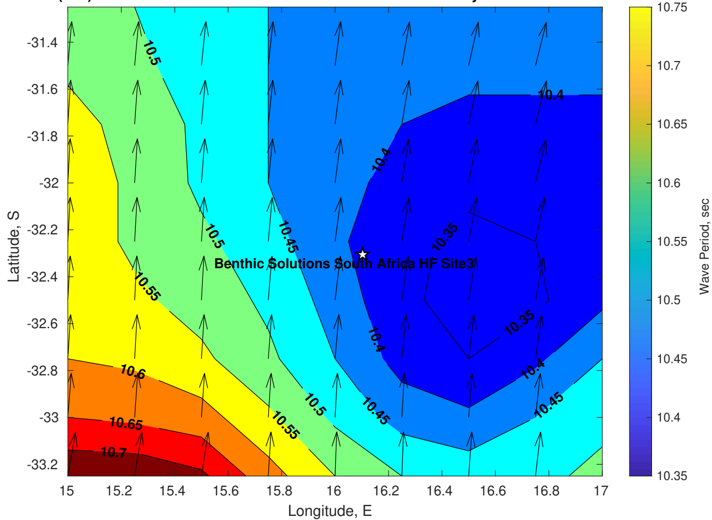
Wave Period (sec) for Benthic Solutions South Africa HF Site3 at 04-May-2025 09:00:00
