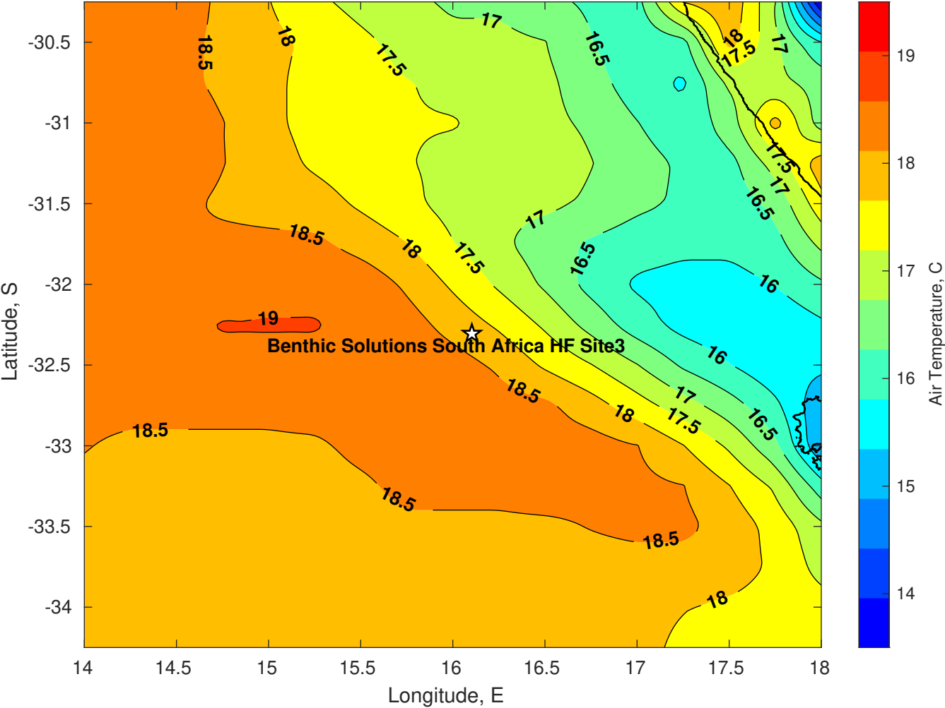
Air Temperature (C) for Benthic Solutions South Africa HF Site3 at 04-May-2025
