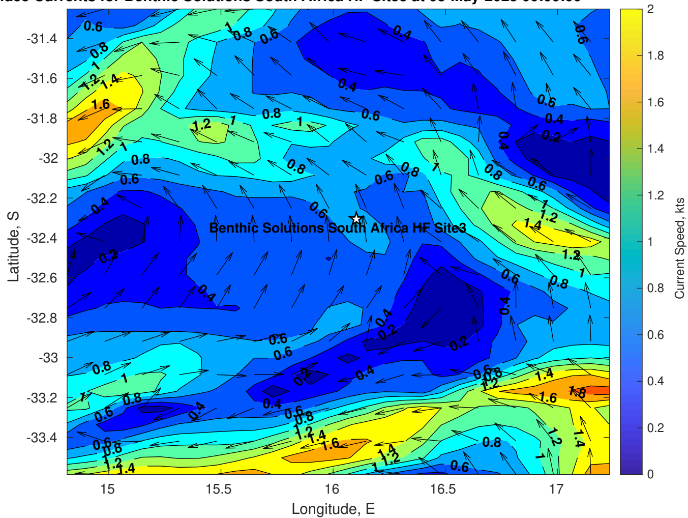
Surface Currents for Benthic Solutions South Africa HF Site3 at 03-May-2025 00:00:00
