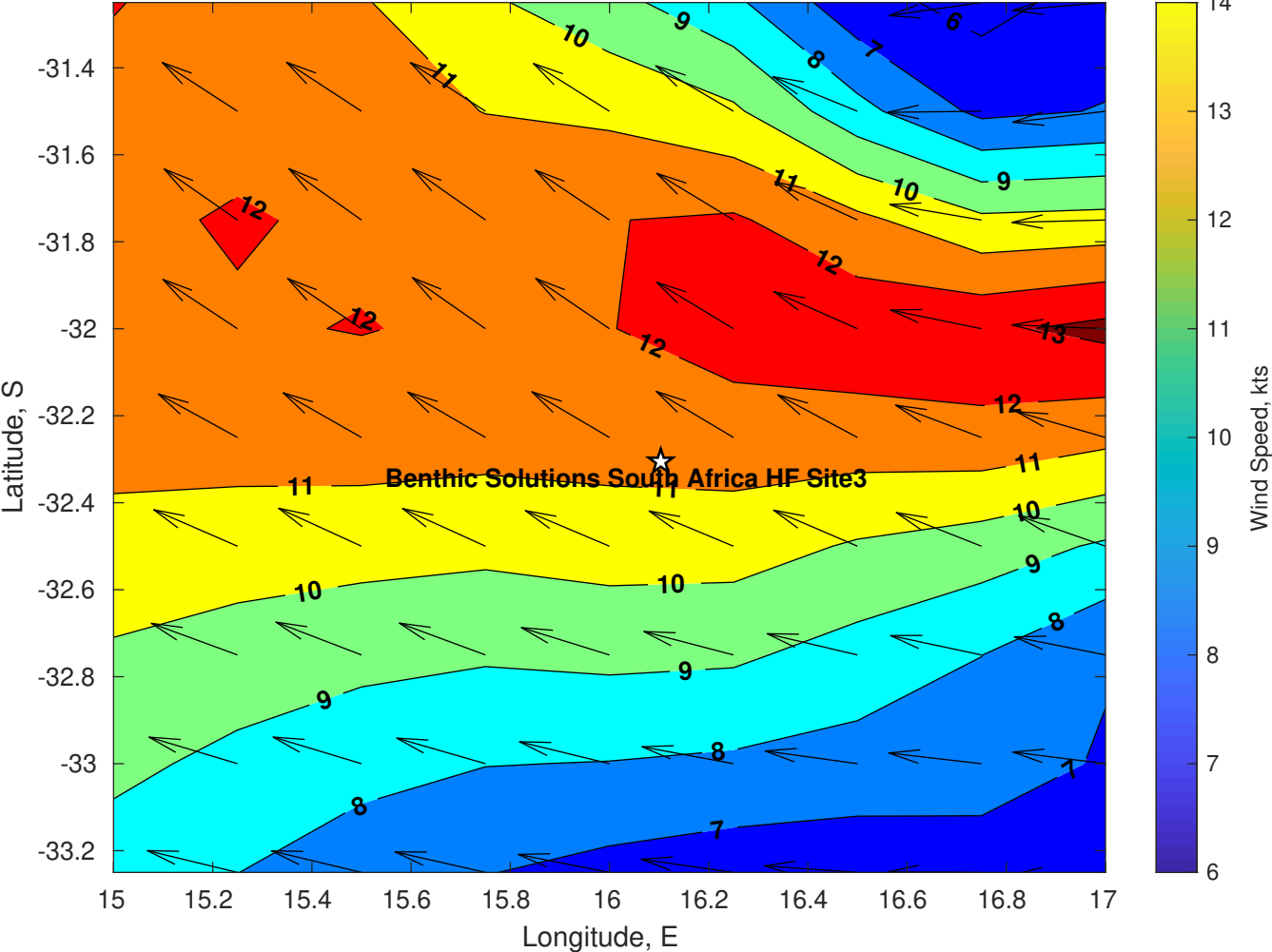
Winds (kts) for Benthic Solutions South Africa HF Site3 at 04-May-2025 09:00:00
