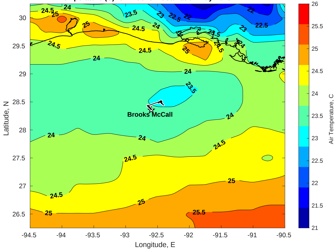
Air Temperature (C) for Brooks McCall at 04-May-2025
