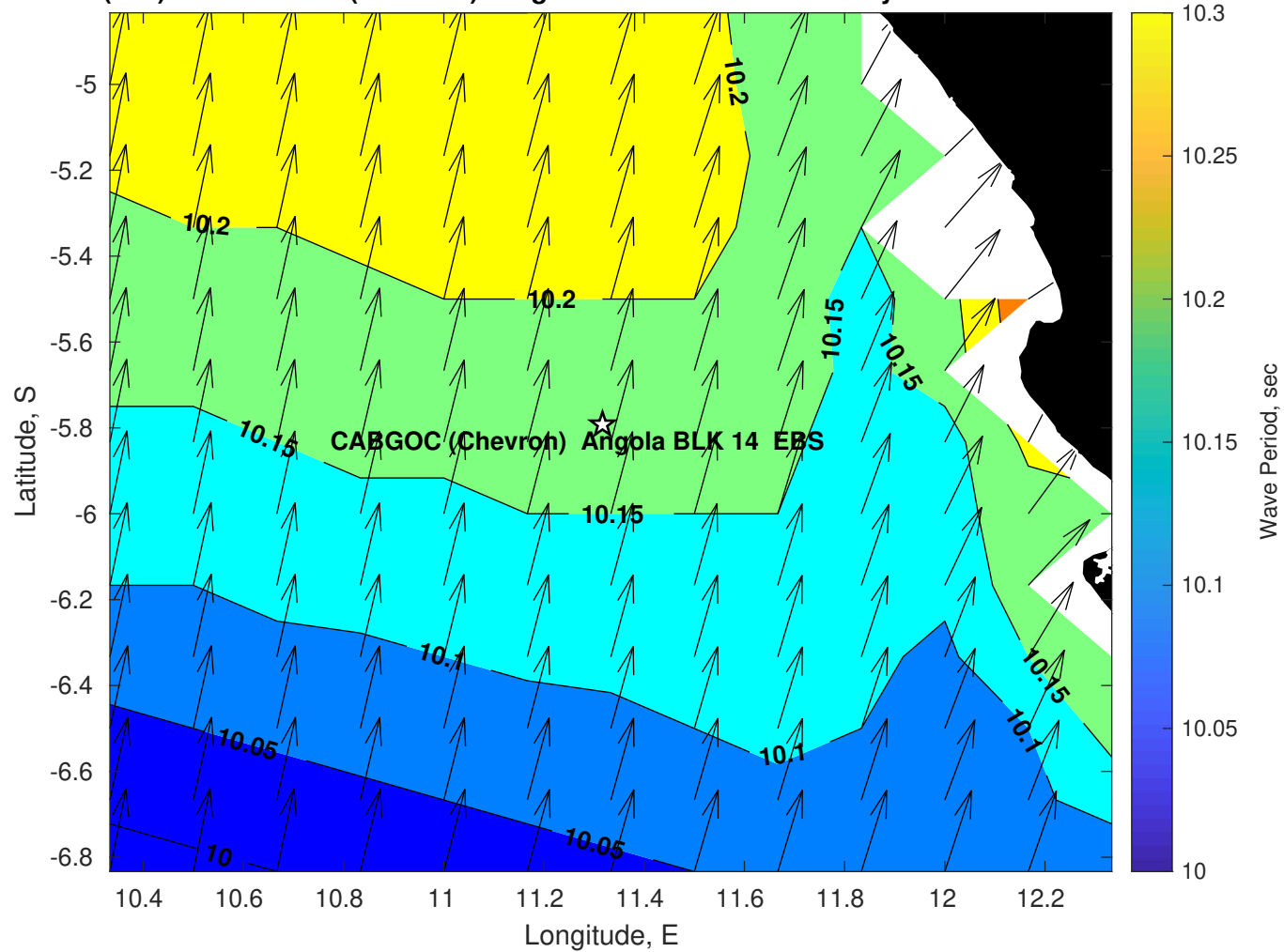
Wave Period (sec) for CABGOC (Chevron) Angola BLK 14 EBS at 04-May-2025 09:00:00
