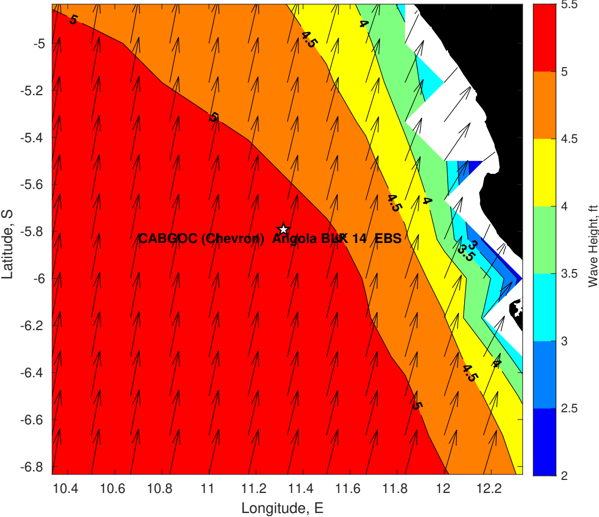
Wave Height (ft) for CABGOC (Chevron) Angola BLK 14 EBS at 04-May-2025 09:00:00
