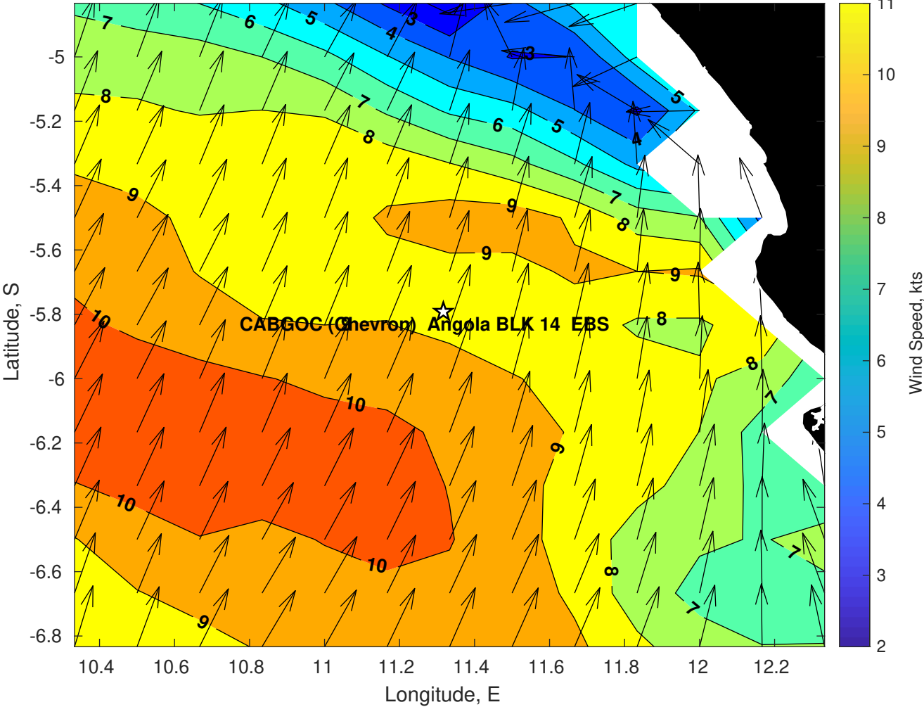
Winds (kts) for CABGOC (Chevron) Angola BLK 14 EBS at 04-May-2025 09:00:00
