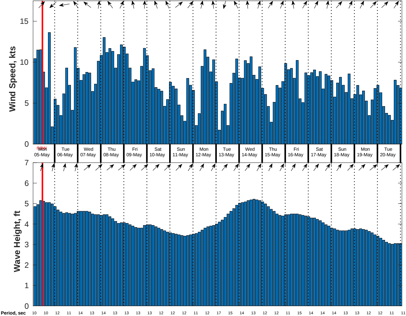
Wind & Wave Forecast for CABGOC (Chevron) Angola BLK 14 EBS from 04-May-2025 02:00:00 to 20-May-2025 02:00:00
