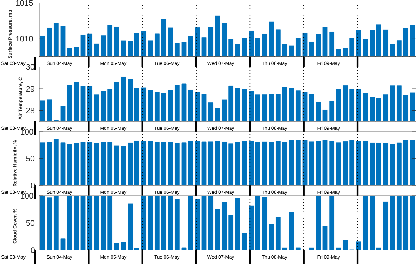
Met Forecast for CSA (ONHYM) PPL EBS - Cote d'Ivoire from 04-May-2025 00:00:00 to 11-May-2025 00:00:00
