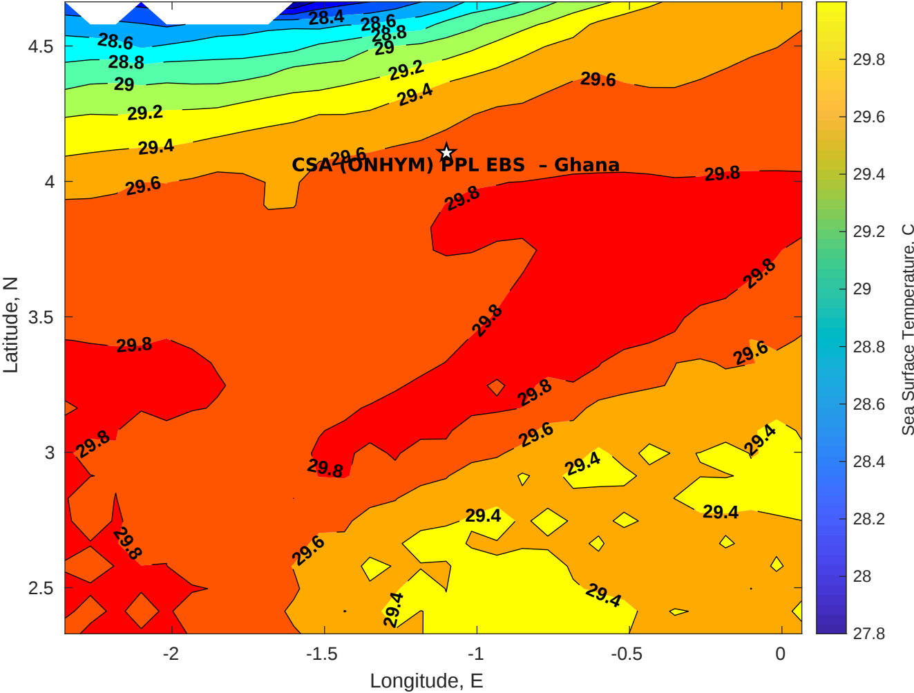
SST for CSA (ONHYM) PPL EBS - Ghana at 03-May-2025 00:00:00
