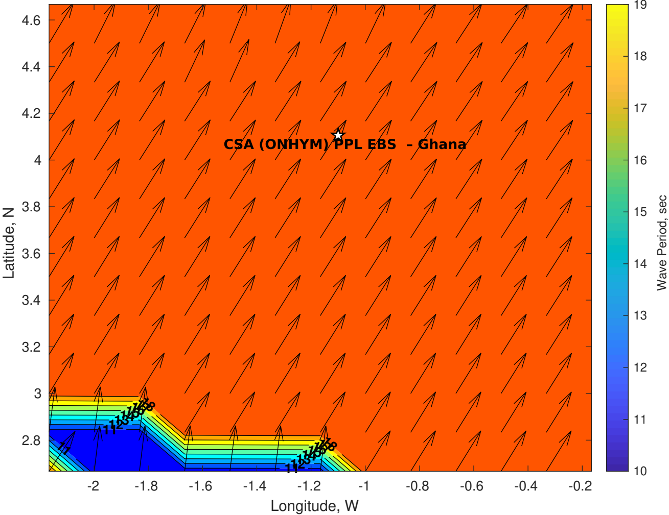
Wave Period (sec) for CSA (ONHYM) PPL EBS - Ghana at 04-May-2025 09:00:00
