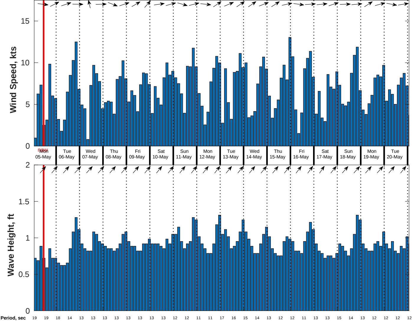
Wind & Wave Forecast for CSA (ONHYM) PPL EBS - Guinea from 04-May-2025 01:00:00 to 20-May-2025 01:00:00
