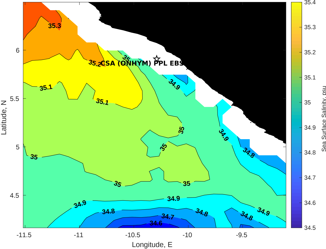
Surface Salinity for CSA (ONHYM) PPL EBS - Liberia at 03-May-2025 00:00:00
