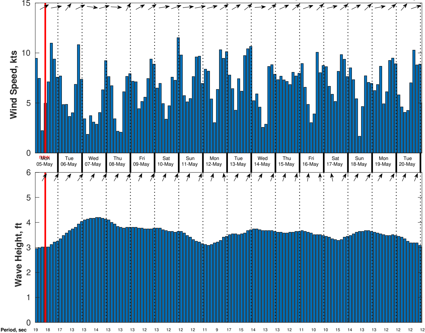
Wind & Wave Forecast for CSA (ONHYM) PPL EBS - Liberia from 04-May-2025 01:00:00 to 20-May-2025 01:00:00
