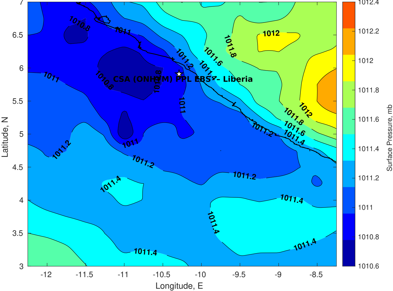
Surface Pressure (mb) for CSA (ONHYM) PPL EBS - Liberia at 05-May-2025 00:00:00
