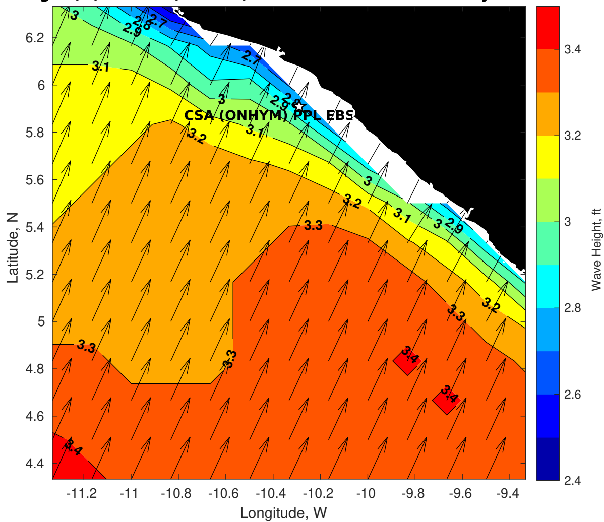
Wave Height (ft) for CSA (ONHYM) PPL EBS - Liberia at 04-May-2025 09:00:00
