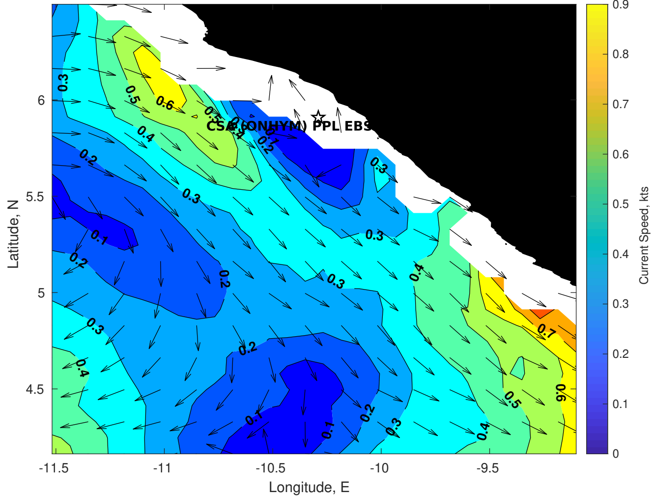
Surface Currents for CSA (ONHYM) PPL EBS - Liberia at 03-May-2025 00:00:00
