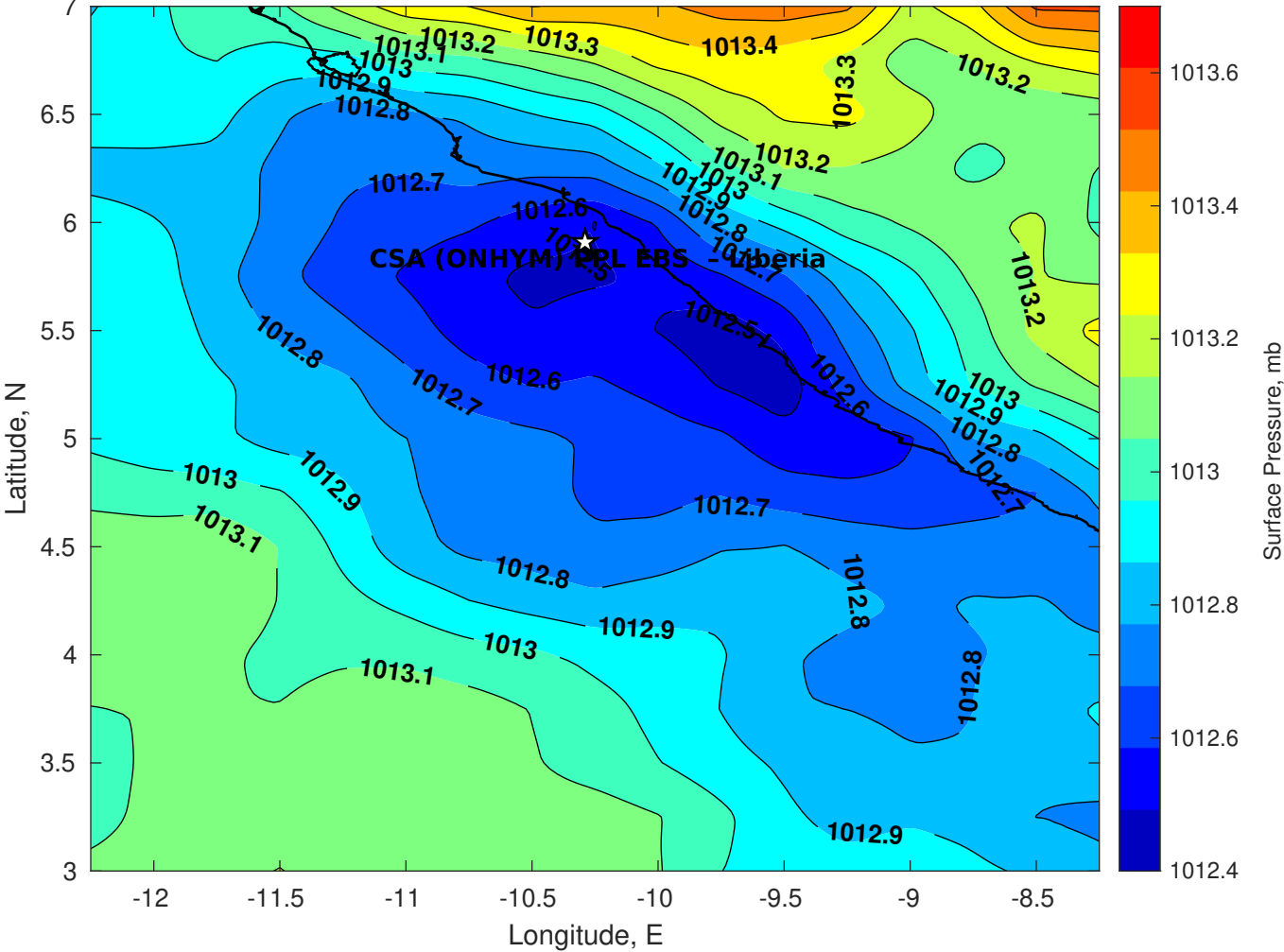
Surface Pressure (mb) for CSA (ONHYM) PPL EBS - Liberia at 04-May-2025 00:00:00
