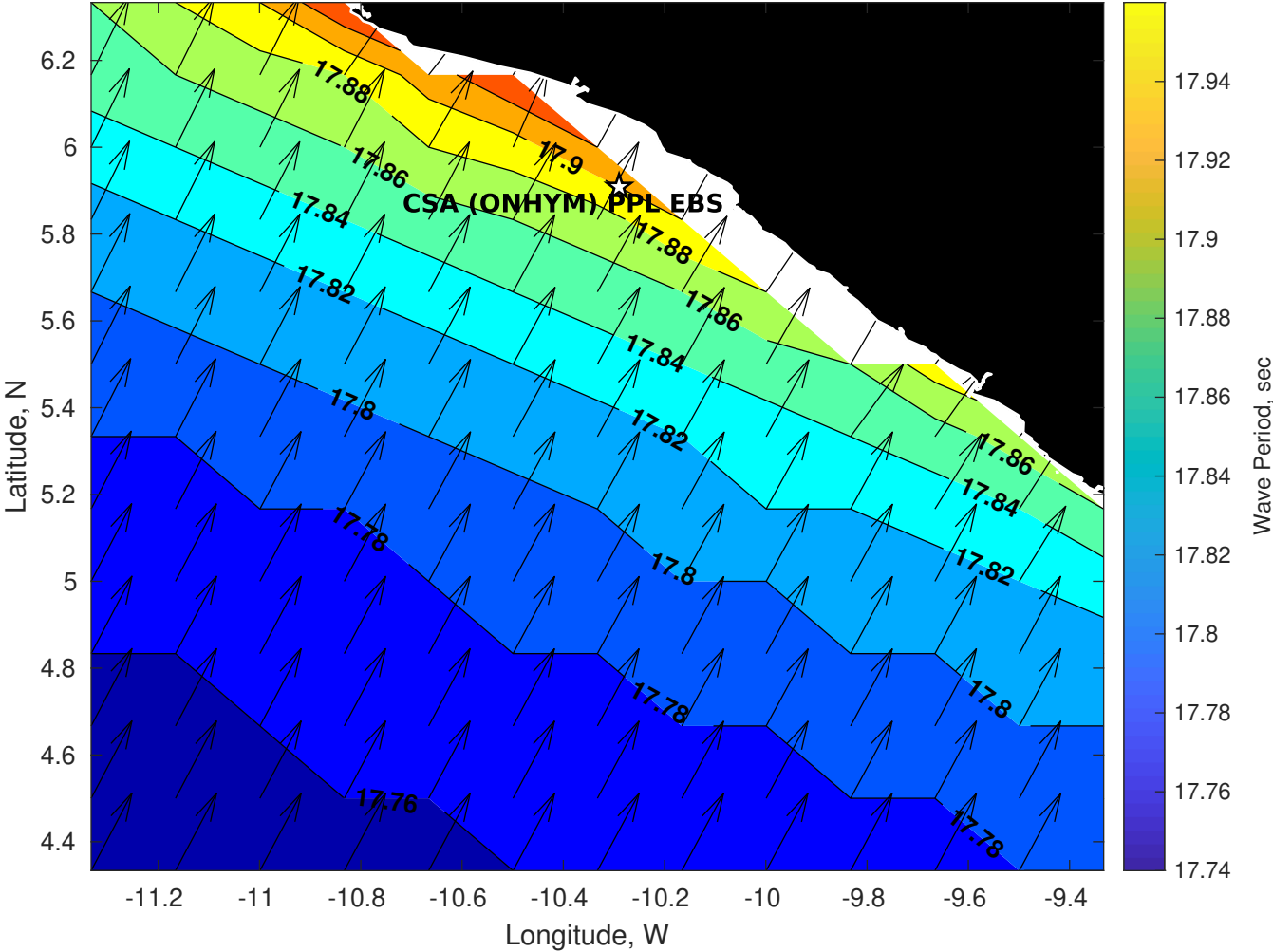
Wave Period (sec) for CSA (ONHYM) PPL EBS - Liberia at 04-May-2025 09:00:00
