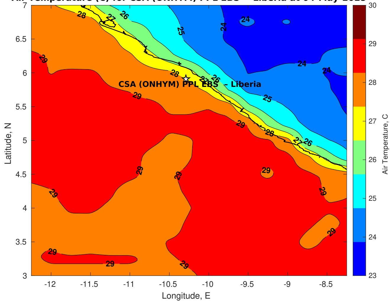
Air Temperature (C) for CSA (ONHYM) PPL EBS - Liberia at 04-May-2025
