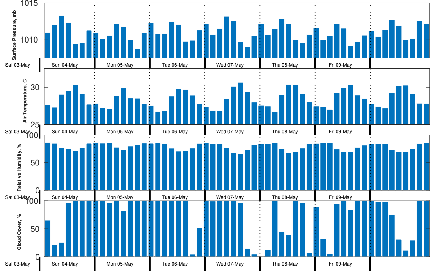
Met Forecast for CSA (ONHYM) PPL EBS - Liberia from 04-May-2025 00:00:00 to 11-May-2025 00:00:00
