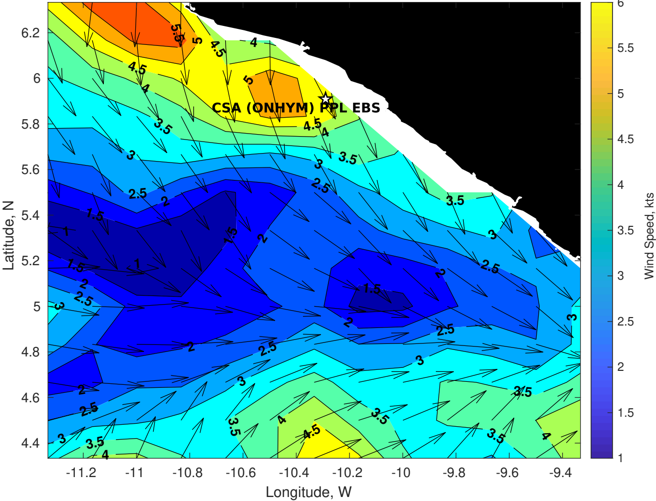
Winds (kts) for CSA (ONHYM) PPL EBS - Liberia at 04-May-2025 09:00:00
