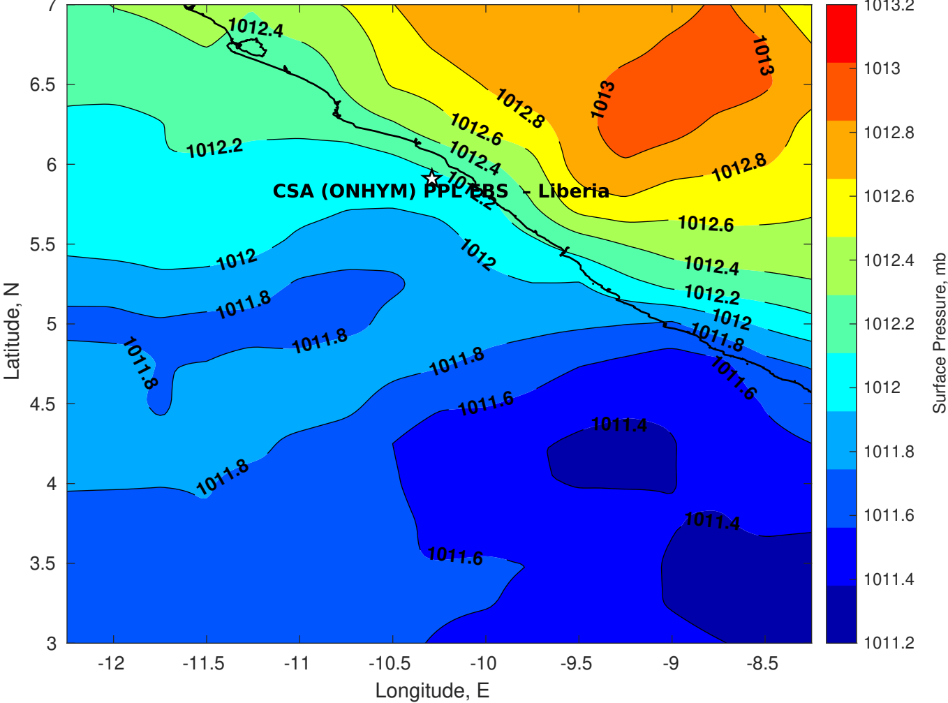
Surface Pressure (mb) for CSA (ONHYM) PPL EBS - Liberia at 06-May-2025 00:00:00
