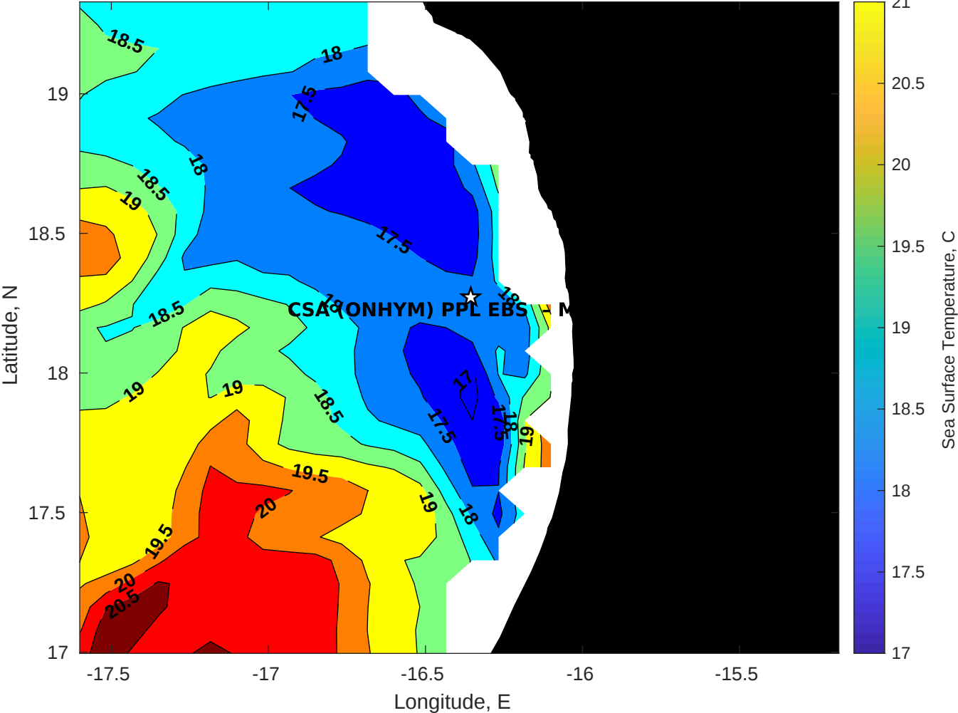
SST for CSA (ONHYM) PPL EBS - Mauritania at 03-May-2025 00:00:00
