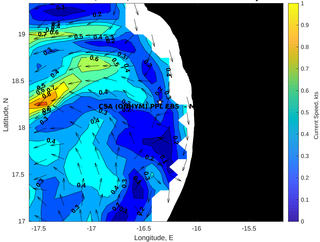
Surface Currents for CSA (ONHYM) PPL EBS - Mauritania at 03-May-2025 00:00:00
