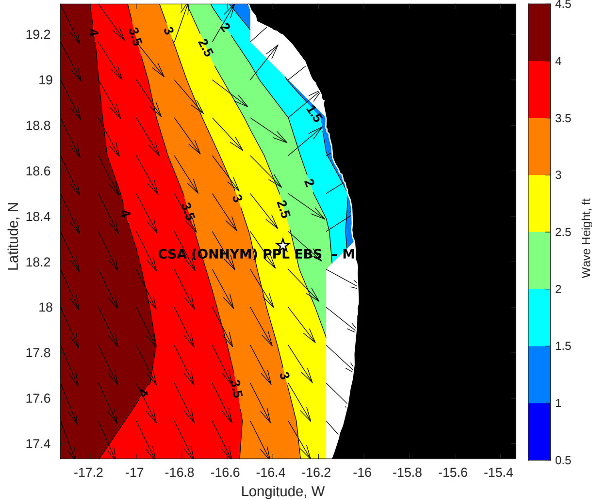
Wave Height (ft) for CSA (ONHYM) PPL EBS - Mauritania at 04-May-2025 09:00:00
