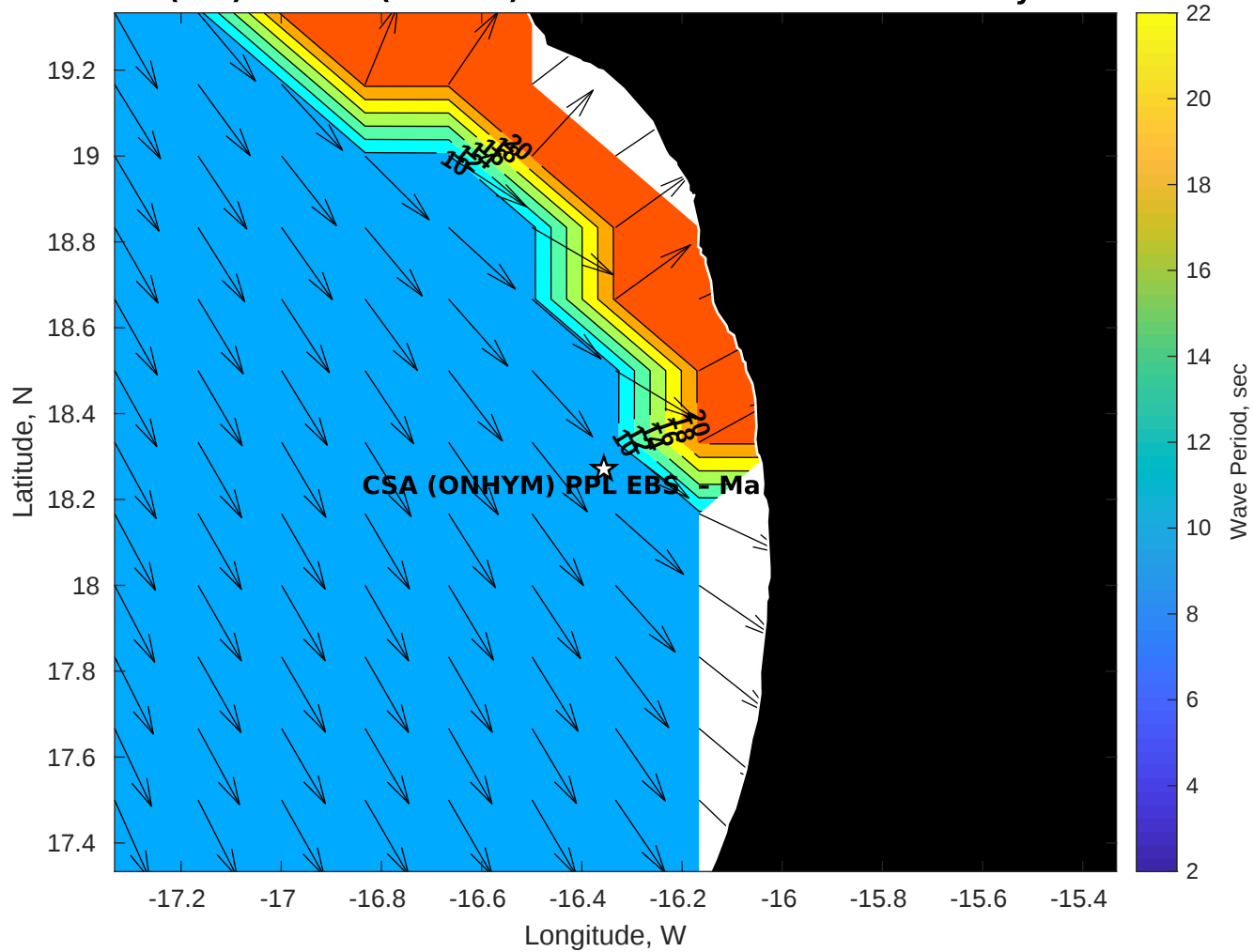
Wave Period (sec) for CSA (ONHYM) PPL EBS - Mauritania at 04-May-2025 09:00:00
