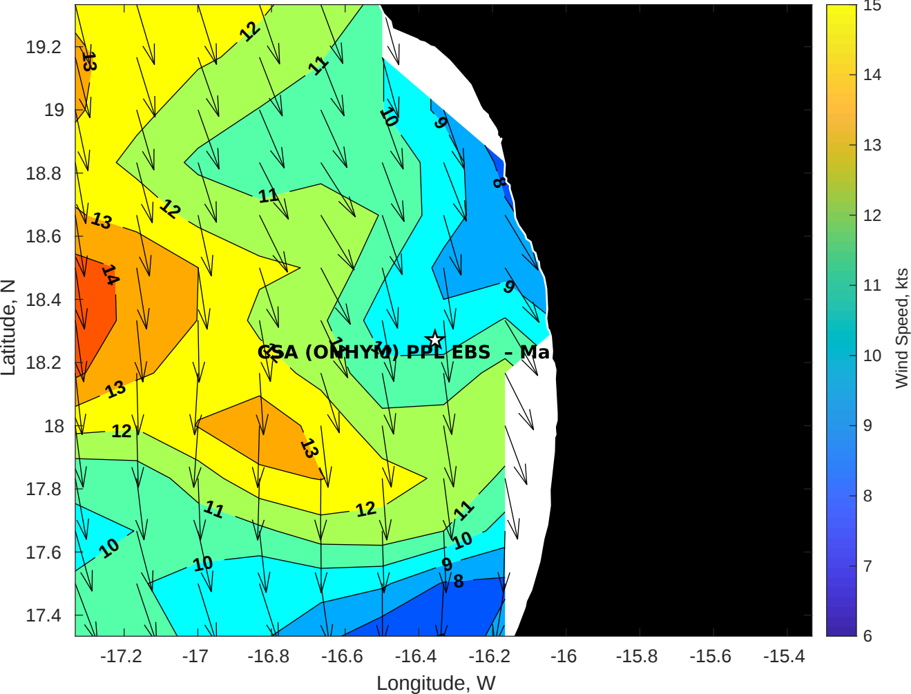
Winds (kts) for CSA (ONHYM) PPL EBS - Mauritania at 04-May-2025 09:00:00
