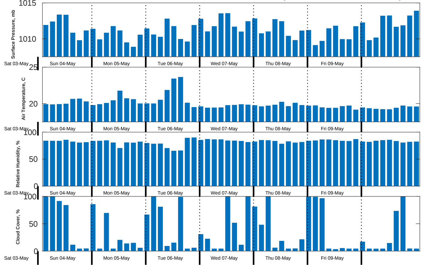
Met Forecast for CSA (ONHYM) PPL EBS - Mauritania from 04-May-2025 00:00:00 to 11-May-2025 00:00:00
